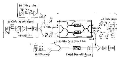
CWD3 Fig. 1. Principle of operation and experimental set-up.
