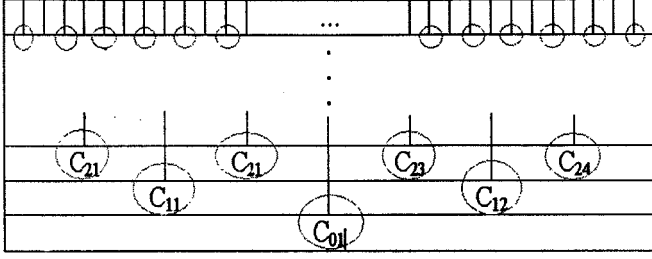
Fig. 4. Structure used in T_{w3} and T_{wc3} to combine three adjacent bins in the wavelet space. Circles illustrate the definitions U_{kj} = C_{kj} + C_{k+1,2j-1} + C_{k+1,2j} .
