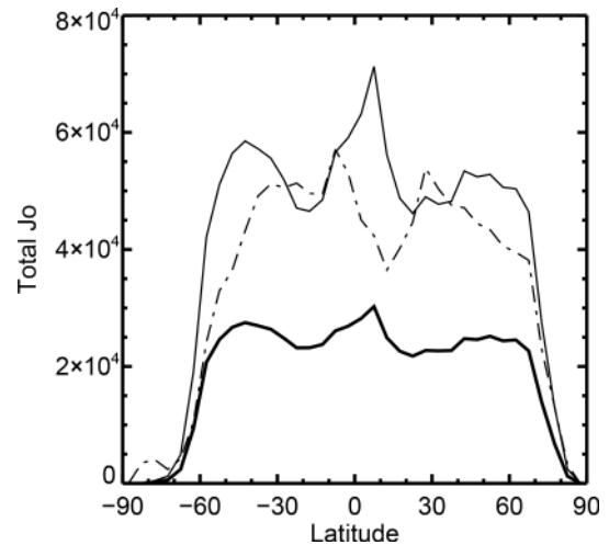
Figure 20. Total of the IASI WV channel contribution to the background observational cost function for Metop-A from 1 to 20 June 2017, accumulated in 5° latitude bins: clear-sky (dotted and dashed line), all-sky before VarQC (thin solid line) and after applying VarQC (thick solid line; this is a hypothetical calculation since VarQC is not applied until later in the minimization).
