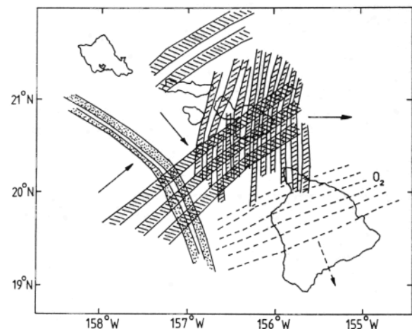
Figure 2. Map showing the geographic positions and scale sizes of the three OI wave motions evident in Figure 1c (assuming an emission height of 96 km). For comparison some of the O 2 data of Figure 1d are also plotted (assuming a height of 94 km).
