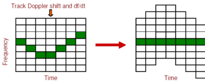
FIG. 2 (color online). An illustration of the discrete frequency bins of the short Fourier transform (SFTs) of the data are shown vertically, with the discrete start times of the SFTs shown horizontally. The dark pixels represent a signal in the data. Its frequency changes with time due to Doppler shifts and intrinsic evolution of the source. By sliding the frequency bins, the power from a source can be lined up and summed after appropriate weighting or transformation. This is, in essence, the starting point for all of the semicoherent search methods presented here, though the actual implementations differ significantly.
