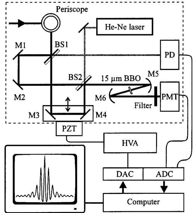
Fig. 9. Schematic of Mach-Zehnder interferometer for measurements of interferometric autocorrelation. BS1, BS2 50% ultra-broadband beam splitters centred at 800 nm; M1–M4 low-dispersion overcoated silver mirrors; M5 r = -10 -cm, unprotected gold coated mirror; BBO 15- \mu\text{m} -thick BBO crystal; M6 r = -10 -cm protected aluminium-coated mirror; PD photodiode; PMT photo multiplier tube; PZT piezo-electric transducer; HVA high-voltage amplifier; DAC digital-analog converter; ADC analog-digital converter. All optics were obtained from R&D Lezer Optika, Budapest
