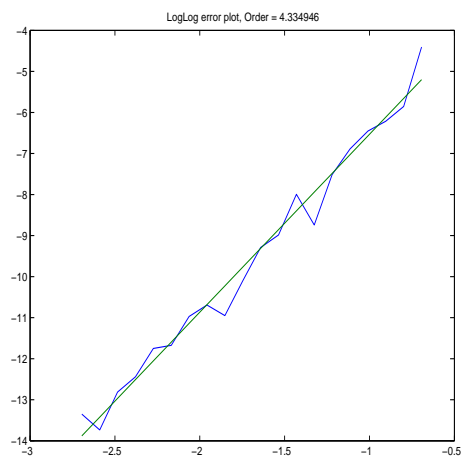
Fig. 1 Errors for Sobolev space H^6 , order \approx 4.3
