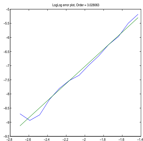
Fig. 2 Errors for C^6 Wendland kernel, order \approx 3
