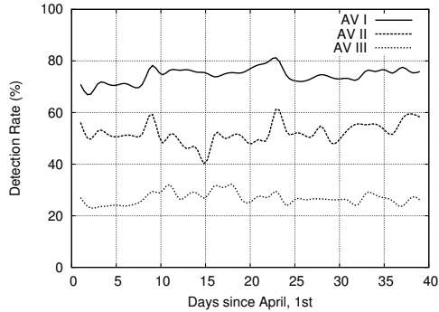
Figure 15: Detection rates of 3 anti-virus engines.
