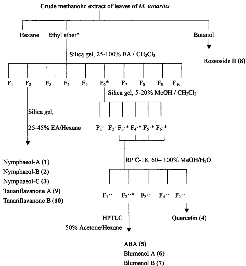
FIG. 2. Scheme for isolating phytotoxic active components from crude methanolic extract of M. tanarius leaves. *High phytotoxic active fraction.
