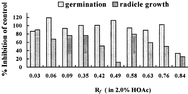
FIG. 6. Chromatographic bioassay of compounds isolated from the ether fraction of aqueous extract of M. tanarius leaves. The corresponding R_f segments of chromatogram with or without spotting extract were used as test and control, respectively. The paper strip was developed with 2.0% acetic acids.
