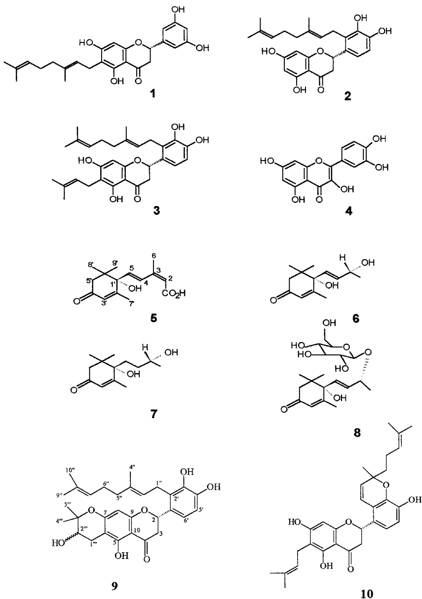
FIG. 7. Chemical structures of the 10 identified compounds from M. tanarius leaves. (1) nymphaeol-A; (2) nymphaeol-B; (3) nymphaeol-C; (4) quercetin; (5) abscisic acid; (6) blumenol A; (7) blumenol B; (8) roseoside II; (9) tanariflavanone A; (10) tanariflavanone B. The compounds are structurally confirmed by ^1\text{H} NMR, ^{13}\text{C} NMR, and MS spectra.
