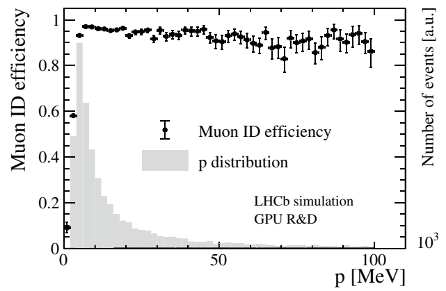
Fig. 9 Muon identification efficiency versus momentum for tracks passing through the Velo, UT and SciFi detectors with respect to all reconstructible muons (explained in the text), for all signal samples combined. The momentum distribution is overlaid as a histogram
