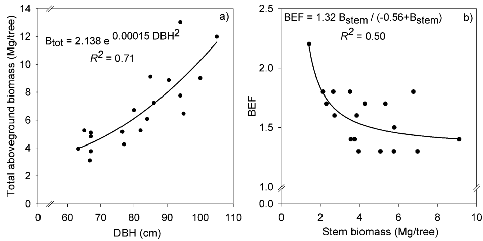
FIGURE 2. Relationship between (a) total aboveground biomass ( B_{tot} ) and DBH (Eq. (11)) and (b) BEF and stem biomass ( B_{stem} ) for sampled trees.
