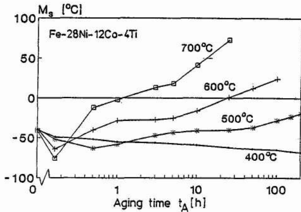
Fig. 10: The effect of ausaging on the martensite start temperature, different ageing temperatures are indicated ( ^{\circ}\text{C} )
