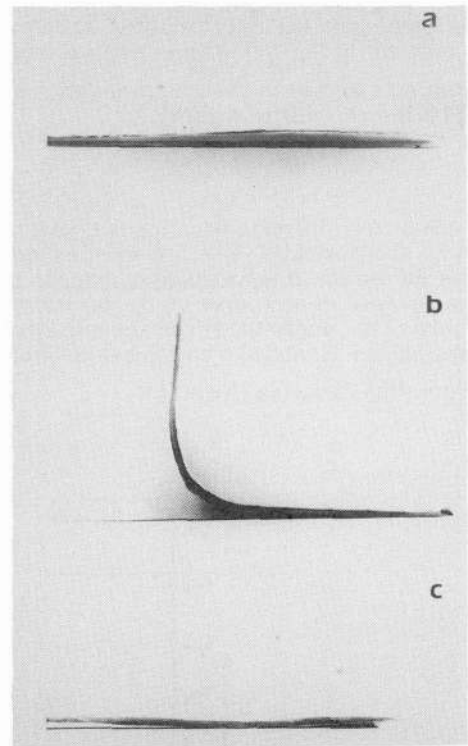
Fig. 5: Shape memory effect in a melt-spun Fe-Mn-Si ribbon
