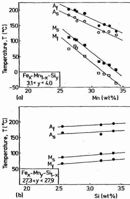
Fig. 4: Influence of Mn- and Si-contents on the transformation temperature in Fe-Mn-Si alloys
