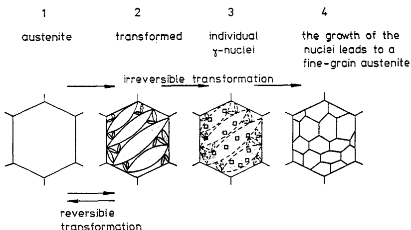
Fig. 3: Two modes of the reformation of austenite: 1) mobile \gamma/\alpha -interfaces \rightarrow reversibility and shape memory; 2) new nucleation of austenite crystals \rightarrow irreversibility
