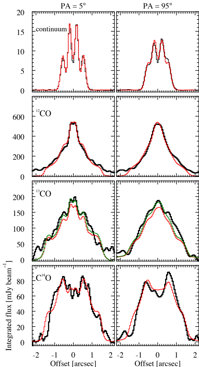
Fig. 7. Results of the fiducial model: comparison of the observed (black curve) and modeled (red curve) radial intensity profiles. In the case of ^{13}\text{CO} , the green curve represents the fiducial model scaled up by 10% to match the absolute flux level.
