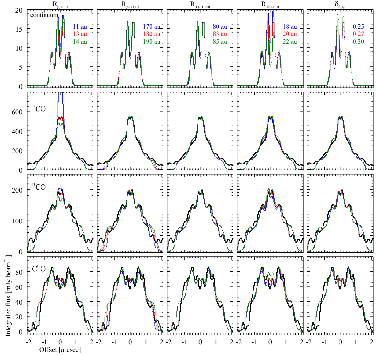
Fig. B.1. Radial intensity profile differences ( \text{PA} = 5^\circ ) for a subset of the model grid. The ^{13}\text{CO} models are scaled up by 10% to match the absolute flux level of the observations.
