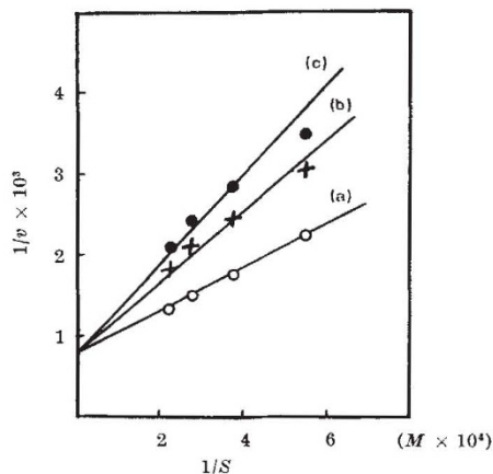
Fig. 2. A Lineweaver and Burk plot of 1/v ( v , \mu l. oxygen/hr./mgm. protein) against 1/S ( S , concentration of cytochrome c ). a , Control; b , with 0.25 ml. of inhibitor; c , with 0.5 ml. of inhibitor prepared as described in the text. Other conditions as in Fig. 1.
