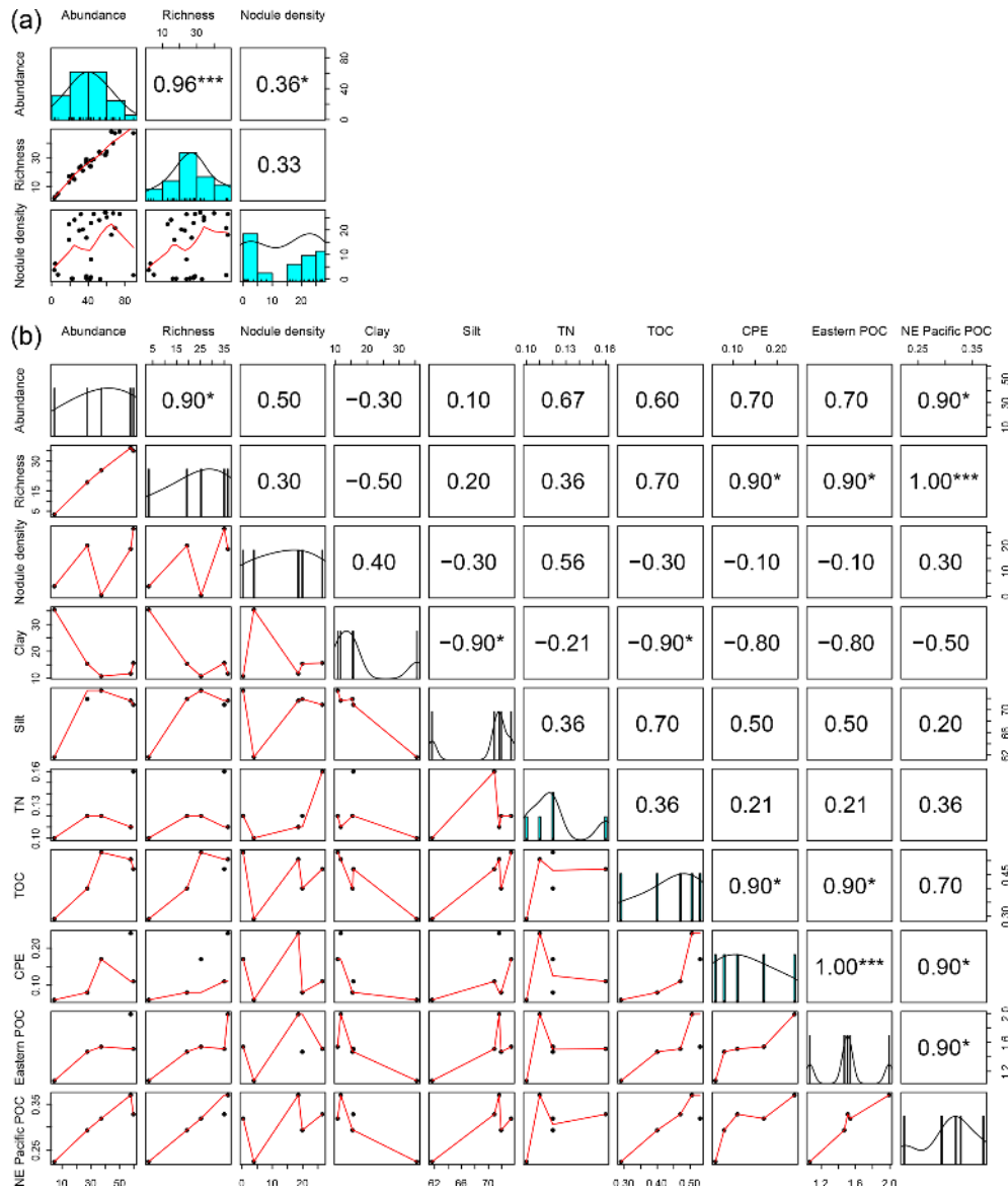
Figure 3. Correlation matrix between biotic and abiotic variables from sampled areas within the eastern CCFZ. Diagonal plots ( a , b ) show the distribution frequency of values for each variable. Panels below the diagonal plots ( a , b ) show the correlation plot between pairs of variables. Panels above the diagonal ( a , b ) plots show the Spearman coefficient correlations between pairs of variables. Abundance, richness and nodule density per box core are shown in ( a ) and average biotic and abiotic variables per area are shown in ( b ). Eastern POC values provided by Volz et al. (2018); NE Pacific POC values were estimated in the present study. * indicates p < 0.05 , ** p < 0.01 and *** p < 0.001 .
