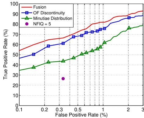
Fig. 20: ROC curves of the proposed algorithm (including three approaches) and NFIQ criterion for detecting altered fingerprints at subject level.
