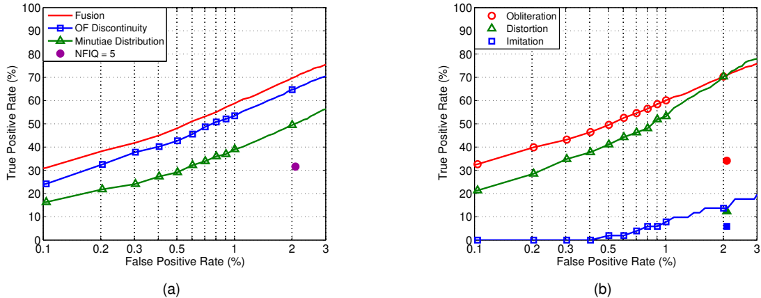
Fig. 16: ROC curves of the proposed algorithm and NFIQ criterion in detecting altered fingerprints. (a) The ROC curves of the three approaches in the proposed algorithm and the NFIQ algorithm and (b) the ROC curves of the proposed fusion algorithm and the NFIQ algorithm for each type of altered fingerprints. The ROC curve of NFIQ criterion is shown as a set of points (only one point is visible in the range of false positive rate plotted here) because its output can only take one of the five quality levels.
