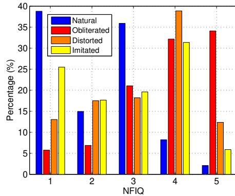
Fig. 12: Histograms of NFIQ values of 27,000 natural fingerprints in NIST SD14 and 4,433 altered fingerprints in our altered fingerprint database according to the type of alteration. Recall that NFIQ = 1 indicates the highest quality.
