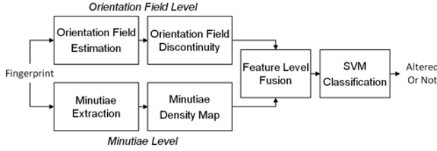
Fig. 13: Flowchart of the proposed algorithm.
