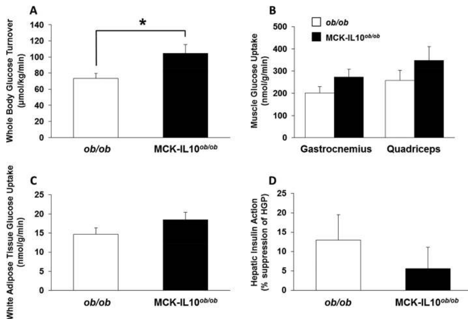
FIG 8 A 2-h hyperinsulinemic-euglycemic clamp in awake MCK-IL10 ob/ob and ob/ob mice. (A) Whole-body glucose turnover in MCK-IL10 ob/ob ( n = 7 ) and ob/ob ( n = 11 ) mice. (B) Insulin-stimulated glucose uptake in gastrocnemius and quadriceps muscles. (C) White adipose tissue glucose uptake in MCK-IL10 ob/ob ( n = 7 ) and ob/ob ( n = 12 ) mice. (D) Hepatic insulin action reflected as insulin-mediated percent suppression of HGP in MCK-IL10 ob/ob ( n = 7 ) and ob/ob mice ( n = 11 ). Values are means \pm SE for each group. *, P < 0.05 .
