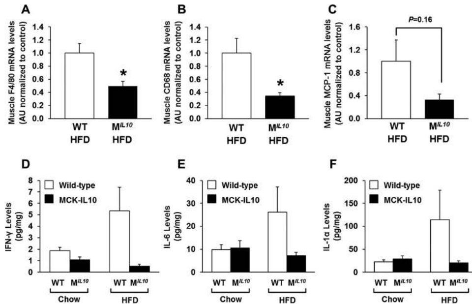
FIG 4 Local inflammation in skeletal muscles of M^{IL10} and WT mice on standard chow or after 16 weeks of an HFD. (A to C) F4/80, CD68, and MCP-1 mRNA levels in quadriceps muscles of HFD-fed M^{IL10} and WT mice as measured by qRT-PCR ( n = 3/\text{group} ). (D to F) IFN- \gamma , IL-6, and IL-1 \alpha levels in gastrocnemius muscles of HFD- and standard-chow-fed M^{IL10} and WT mice as measured by multiplex ELISA ( n = 4 to 6/\text{group} ). Values are means \pm SE for each group. *, P < 0.05 . AU, arbitrary units.
