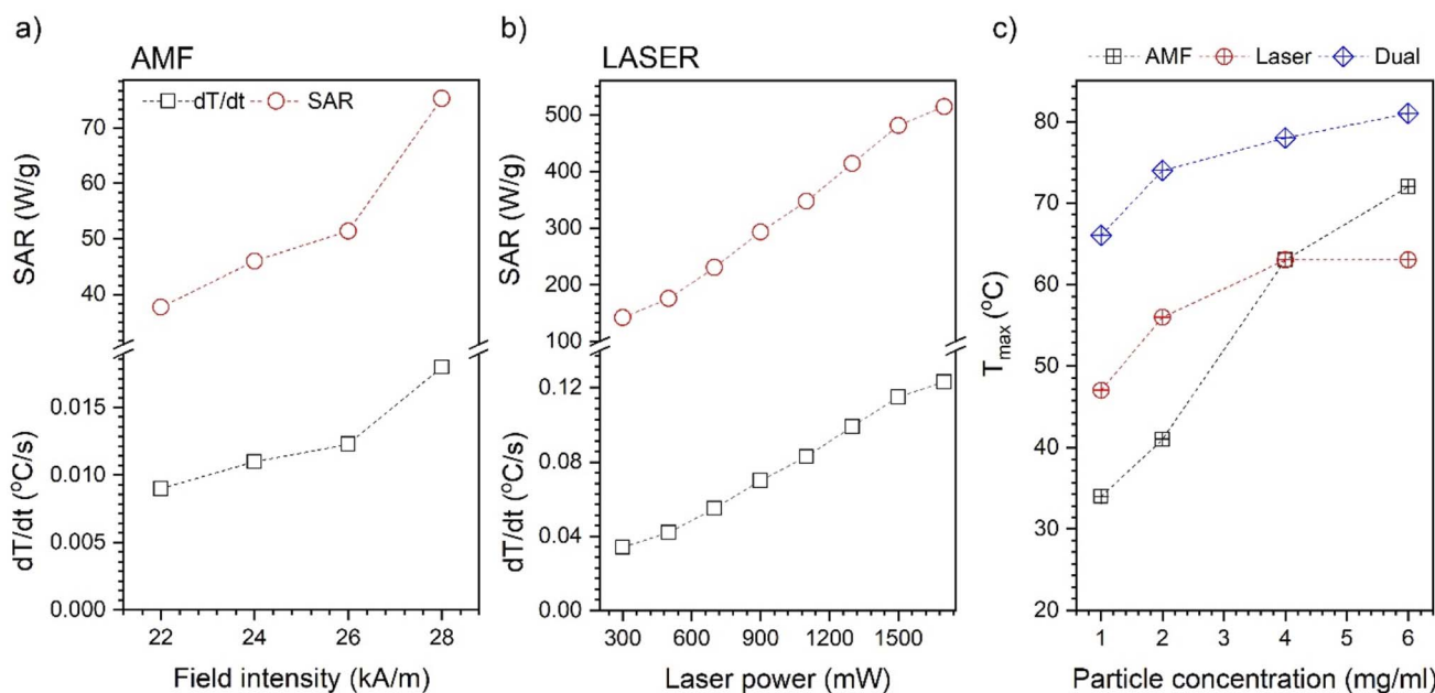
Fig. 8 Dependence of the magnetic field intensity (a) and laser power (b) on SAR and dT/dt values. Plot (c) shows nanoparticle concentration dependence on the T_{max} under different stimulation modes.
