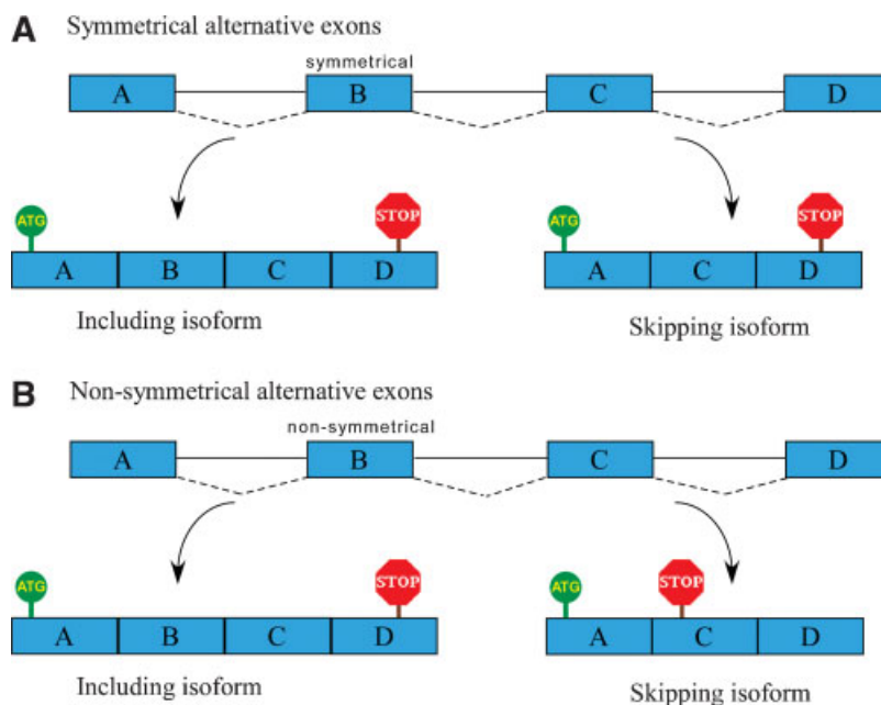
Figure 4. Effects of symmetrical and non-symmetrical alternatively spliced exons on the reading frame. A: A schematic of a gene structure consisting of four exons, where the second exon is a symmetrical cassette exon, is depicted. Inclusion or exclusion of the symmetrical exon does not alter the open reading frame of the downstream exons. B: A gene consisting of four exons, where the second exon is a non-symmetrical cassette exon, is illustrated. Inclusion or exclusion of the non-symmetrical exon results in a frame-shift and a PTC downstream of the alternative exon.
