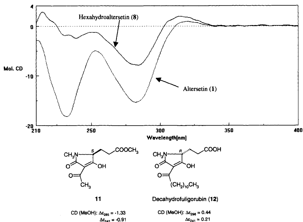
Fig. 7. CD data ( \Delta\epsilon [ \text{cm}^2 \cdot \text{mmol}^{-1} ]) of compounds 1 and 8 in MeOH and reference CD data of tetramic acids. 17)
