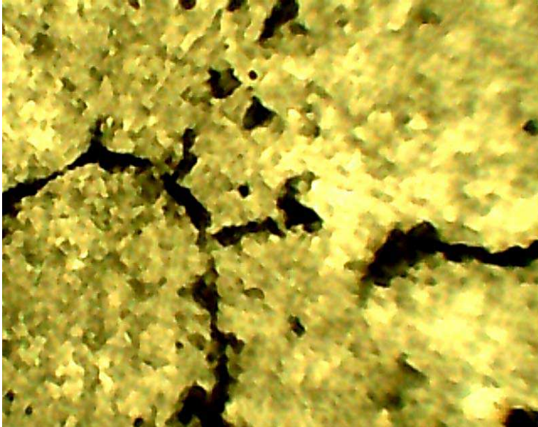
Fig. 11. Countergravity cast specimen at 400× magnification. Significant reduction of impurities at the gain boundaries indicates lesser intake of impurities from the melt
