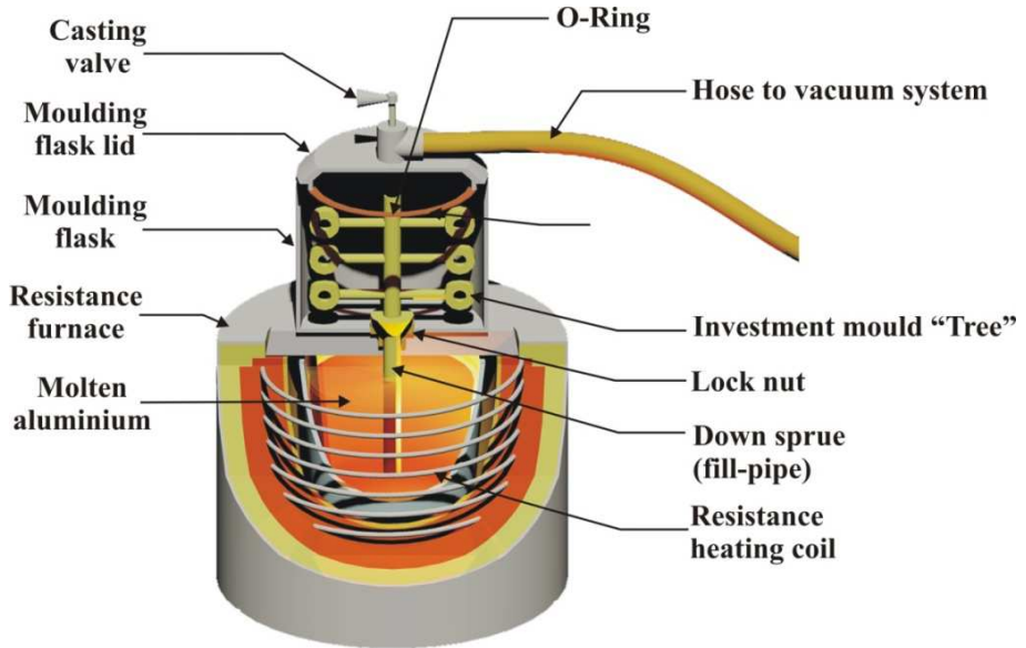
Fig. 1. Typical setup of the countergravity casting process
