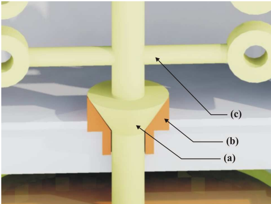
Fig. 2. Down sprue, with conical base (a) is integrated with the rest of the investment mould "tree" (c). The assemble rests inside the conical depression of the lock-nut (b)
