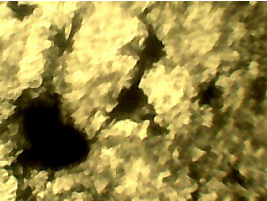
Fig. 6. Gas porosity in aluminium casting at 1000× magnification
