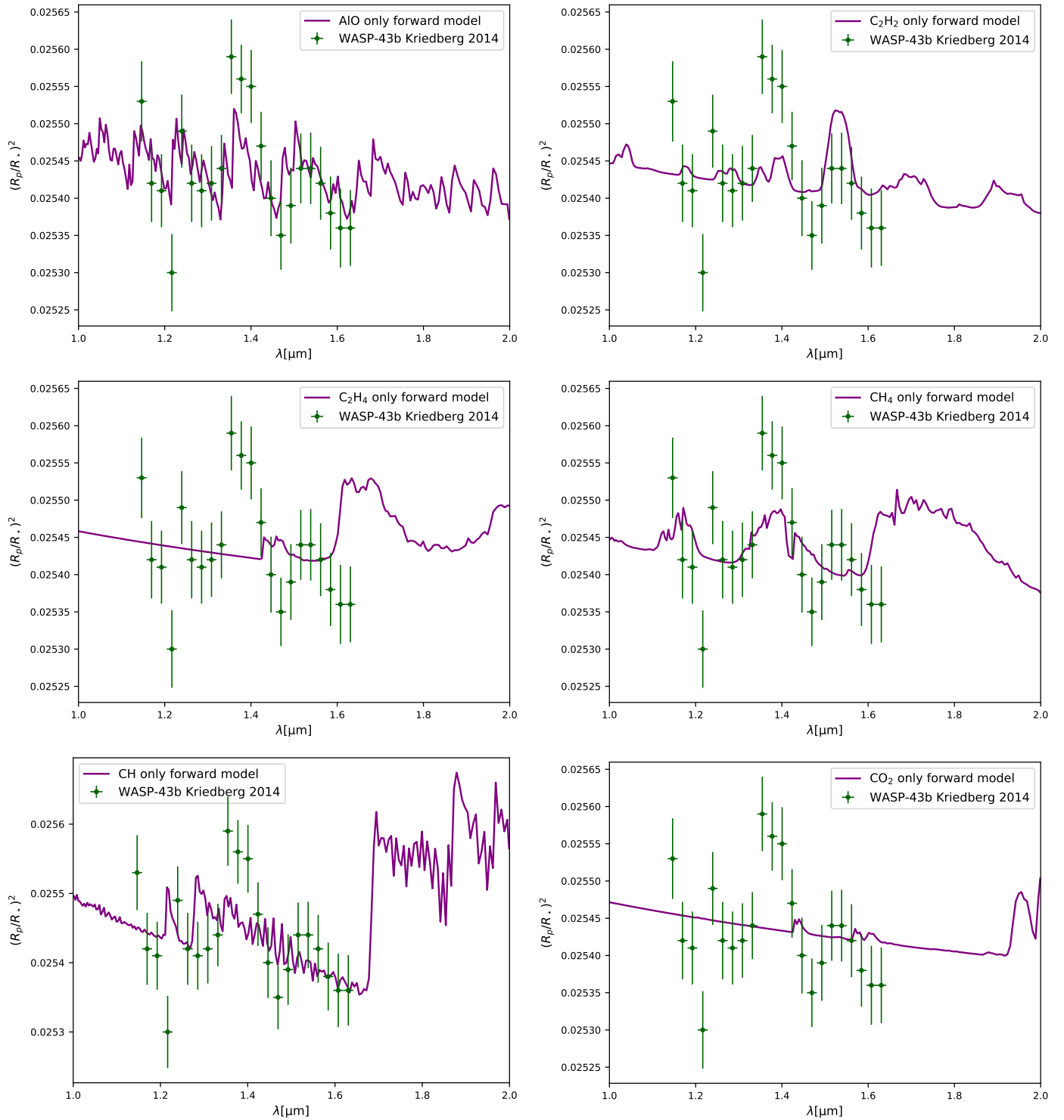
Fig. B.1. ARCiS forward models, each including one individual species, plotted alongside the transmission data for WASP-43b from Kreidberg et al. (2014) in order to help assess which molecules to include in subsequent retrievals.
