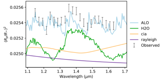
Fig. 2. Contributions of molecular features to the cloud-free Tau-REx retrieval results that include AlO and H 2 O only.
