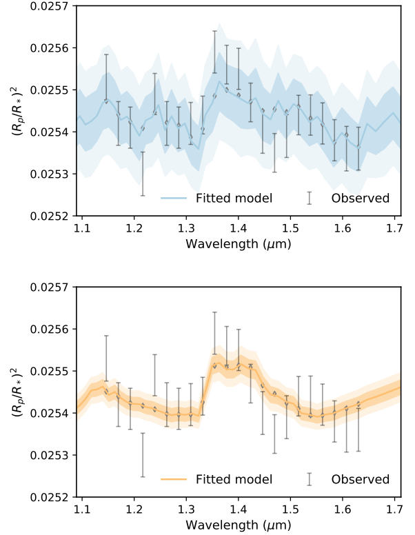
Fig. 1. Cloud-free Tau-REx transmission retrieval results with H 2 O and AlO (top) and with H 2 O only (bottom). The different shading corresponds to 1\sigma and 2\sigma regions.
