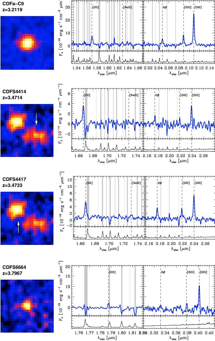
Fig. 1. [OIII]5007 line maps ( left ) and near-IR spectra ( right ) of the galaxies in the AMAZE sample presented here. Each [OIII]5007 map has a size of 3'' \times 3'' . The vertical dotted lines in the spectra indicate the expected location of nebular emission lines. The bottom panels show the sky spectrum. The shaded vertical regions overlaid on each spectrum highlight spectral region affected by strong sky emission lines.
