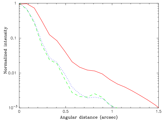
Fig. 5. Azimuthally averaged intensity profile of L 2 Pup (red solid line) and the PSF references \epsilon Cru (green dashed line) and S Ori (blue dotted line). The central region of L 2 Pup within 0''.1 is saturated.
