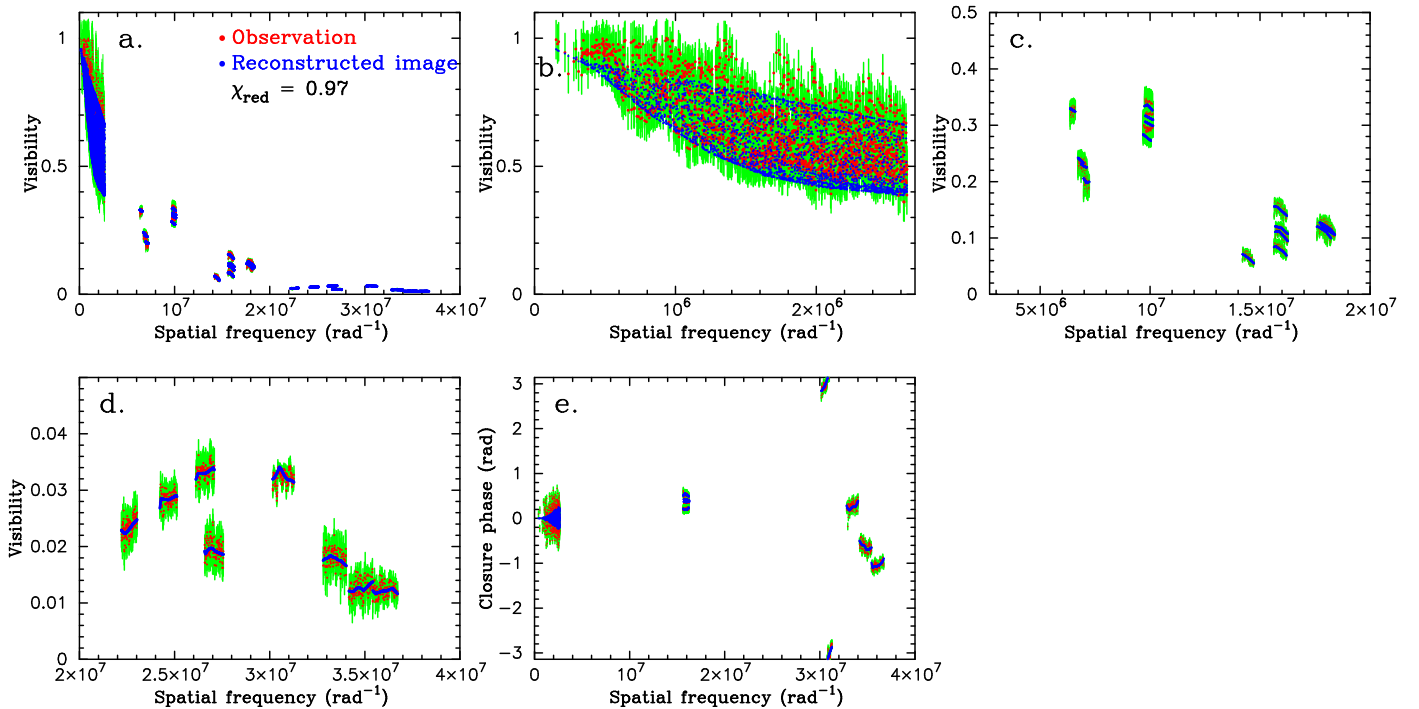
Fig. 3. Comparison of the observed interferometric data and the corresponding observables from the reconstructed image shown in Fig. 2b. The observed data are plotted with the red (black in the printed edition) symbols with the error bars shown in green (light gray), while the model is represented by the blue (dark gray) symbols. a) Visibilities. b) Enlarged view of the visibilities obtained by speckle interferometry with NACO. c) and d) enlarged views of the visibilities obtained with AMBER in two different spatial frequency ranges. e) Closure phases.
