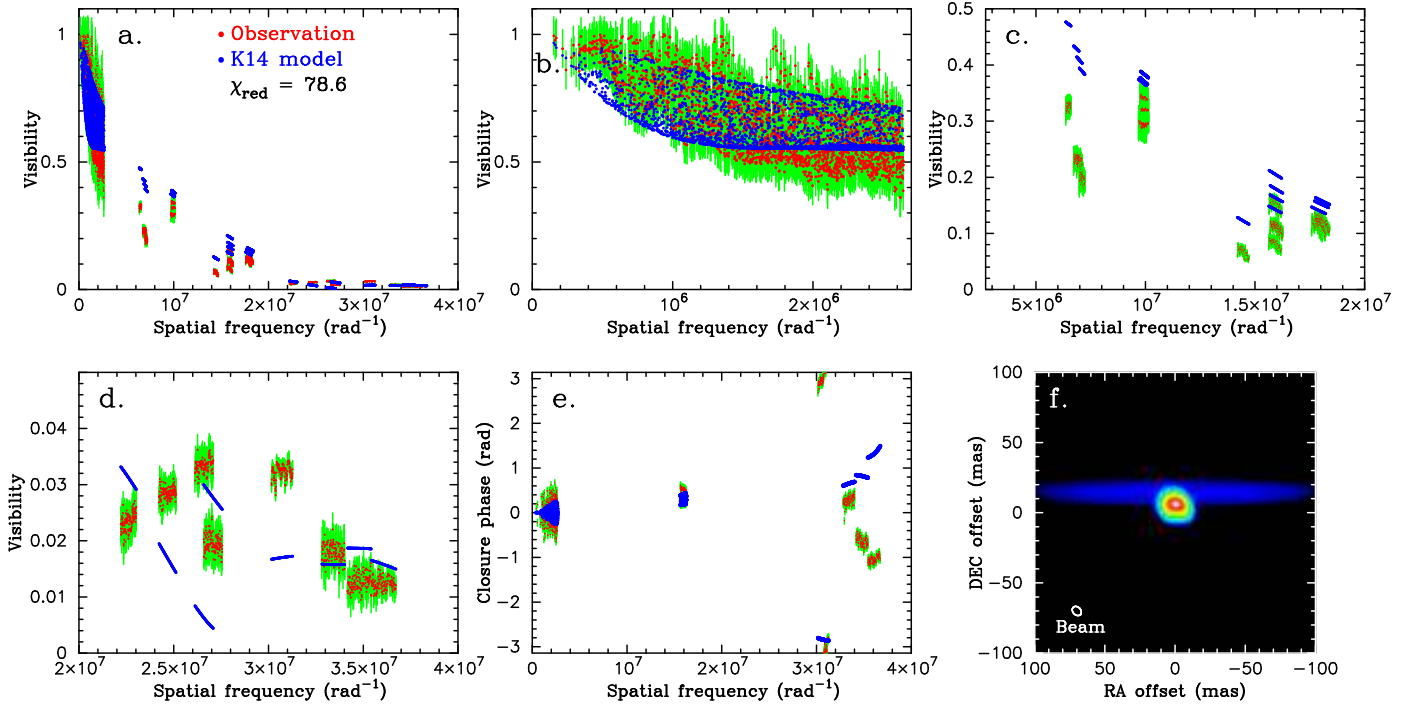
Fig. 6. Comparison of our NACO speckle and AMBER observations with the RT model of K14. In panels a)–e) , the observed data are plotted with the red (black in the printed edition) symbols with the error bars shown in green (light gray), while the model is represented by the blue (dark gray) symbols. a) Visibilities. b) Enlarged view of the visibilities obtained by speckle interferometry with NACO. c) and d) enlarged views of the visibilities obtained with AMBER in two different spatial frequency ranges. e) Closure phases. f) Model image in the same color scale as the reconstructed images in Fig. 2.
