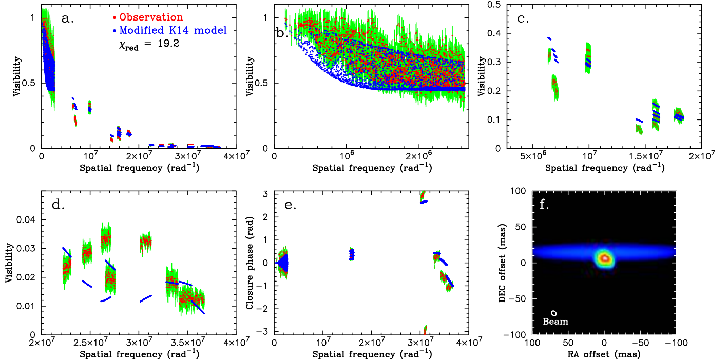
Fig. 7. Comparison of our NACO speckle and AMBER observations with the modified RT model of K14, shown in the same manner as in Fig. 6.
