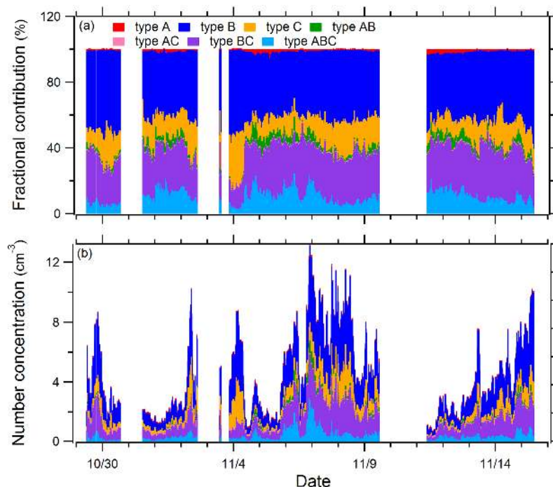
Figure 4. Time series of (a) the fractional contribution of each fluorescent type to total FAPs and (b) number concentration (left axis) of each fluorescent type. Type A: red; type B: blue; type C: dark yellow; type AB: green; type AC: pink; type BC: purple; type ABC: light blue.
