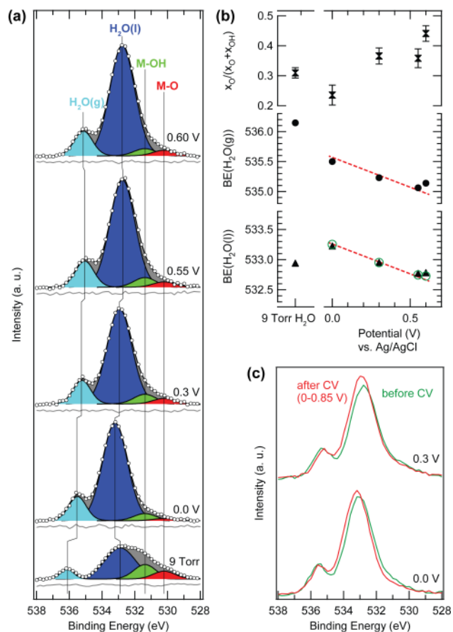
Figure 2. (a) Normalized and background-subtracted O1s XPS spectra of Ni-Fe (7 nm) electrocatalyst, excited with 4020 eV X-ray photons. Bottom to top: as-prepared catalyst exposed to 9 Torr H 2 O pressure, and operando measurements, taken after extended electrochemical conditioning (6 cycles, 0-0.65 V, and 6 cycles, 0-0.85 V) under a ~30 nm thick 0.1 M KOH liquid film at the indicated applied potentials (vs. Ag/AgCl). The measured spectra (circles) are
