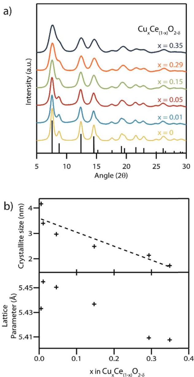
Fig. 4 (a) Synchrotron X-ray diffraction patterns of the as-synthesized \text{Cu}_x\text{Ce}_{1-x}\text{O}_{2-\delta} materials with varying Cu content showing good agreement with the \text{CeO}_2 fluorite structure, space group \text{Fm}\bar{3}\text{m} (ICSD collection code 156250, reference peak positions shown). The progressive broadening of the peaks with increasing copper content is indicative of decreasing crystallite mean size. The trend line is provided as a guide to the eye. (b) Lattice parameter and crystallite size measurements derived from Rietveld refinement of the XRD patterns presented in (a).
