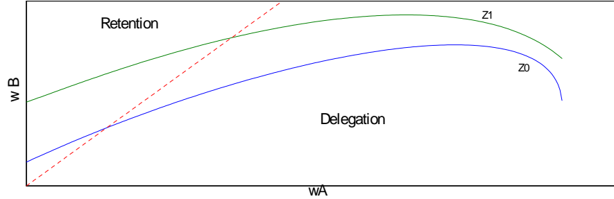
Figure 1: Indifference Curve for Outside Portfolio. The solid lines plot the indifference curve between delegation and retention for different levels of productivity, Z . The dotted line plots w_B = w_A + (1 - \alpha) V_A . An increase in w_B causes retention to be more attractive, while an increase in w_A is non-monotonic, favoring first delegation and then retention. When Z is larger, this cutoff increases: Z1 > Z0 .
