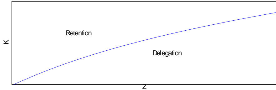
Figure 2: Indifference Curve for Productivity, Z , and Outside Portfolio, K . Increasing the outside portfolio of outsiders, K (where w_A = K - (1 - \alpha) V_A and w_B = K ), makes retention more attractive, but increasing the growth options, Z , makes delegation more attractive.
