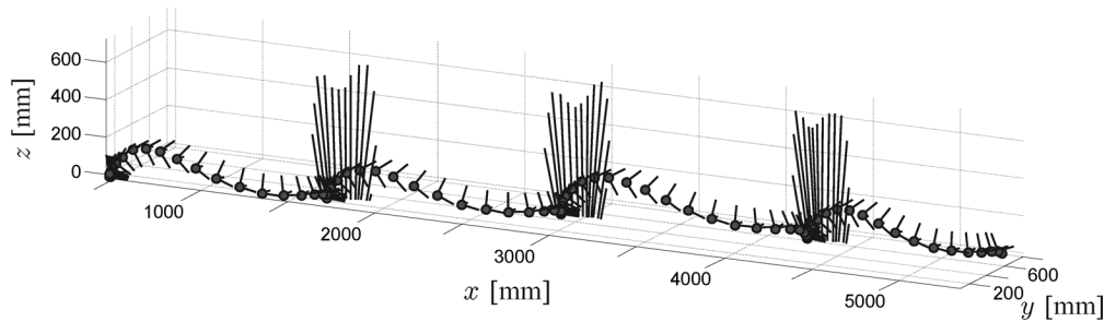
Fig. 7. CoP, GRF, position, and orientation of the heel sensor during several steps. The CoP and GRF of three steps are indicated by the lines pointing upwards. The position of the heel sensor is indicated by the dots, the corresponding orientation by the three lines representing the heel sensor coordinate axes.
