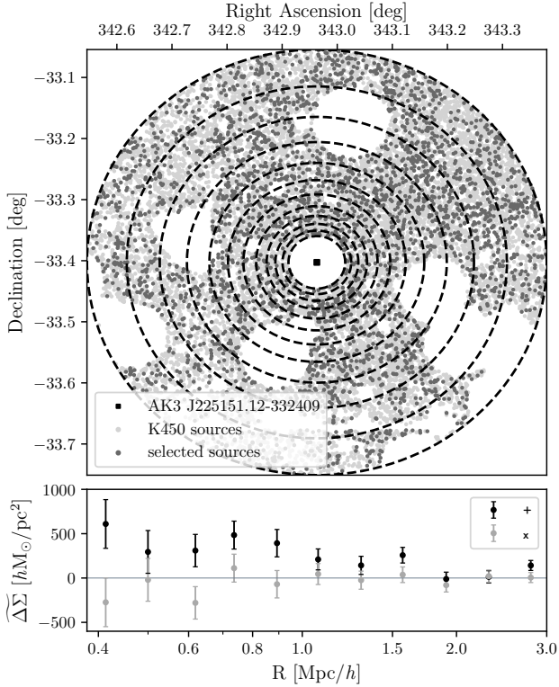
Figure 2. Top panel: Illustration of eleven of the thirty annuli in the radial range [0.35, 3] Mpc/h, for the cluster AK3 J225151.12-332409. The sources shown are selected following the cut discussed in Section 3.3.1. Blank regions indicate masks (Hildebrandt et al. 2017). Bottom panel: Tangential and cross components of the excess surface mass density (Equation 8) of J225151.12-332409. Vertical error bars are derived from Equation (11).
