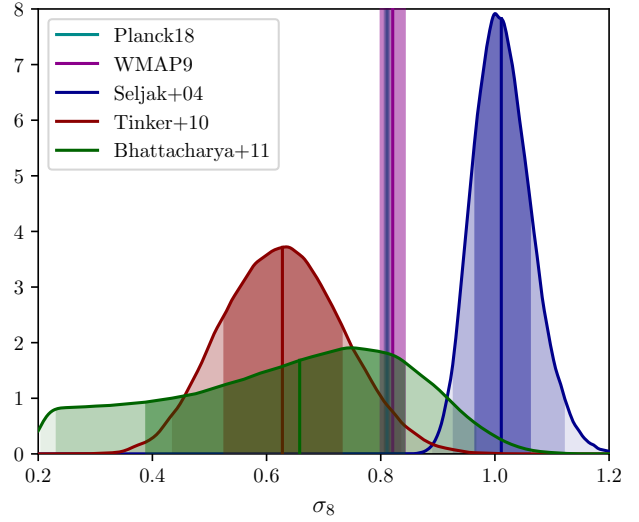
Figure 10. Posterior distribution for \sigma_8 . The probability function is shown for three halo bias-mass relations, i.e. Seljak & Warren (2004), Tinker et al. (2010) and Bhattacharya et al. (2011), shown in blue, red and green, respectively. The dark to light shaded regions correspond to the 1 – 2 – 3 \sigma intervals. We compare these distributions with the median values of Planck (cyan, Planck Collaboration et al. 2020, Table 2, TT,TE,EE+lowE+lensing) and WMAP (magenta, Hinshaw et al. 2013, Table 3, WMAP-only Nine-year).
