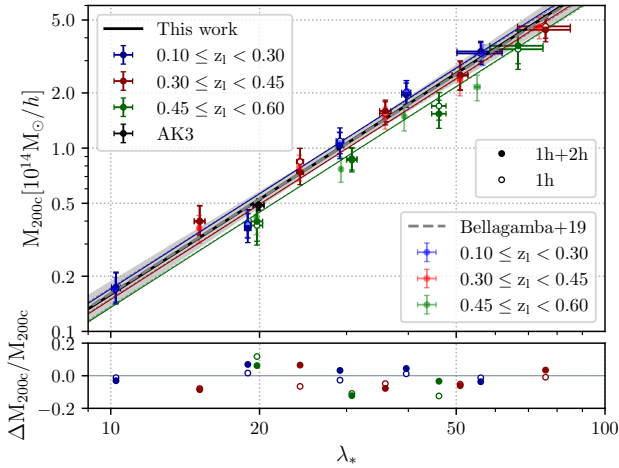
Figure 7. Mass-richness scaling relation for the full catalog (black) and for the low (blue), intermediate (red) and high (green) redshift bins. The thick line corresponds to the model formulated in Equation (36). Full and empty data points represent the measurements over the whole radial profile and over the central region of the halo, respectively. We compared our results with those presented in Bellagamba et al. (2019). The fainter colored points represent the data and the dashed lines represent the model. The relative change with respect to the results of this work is displayed in the bottom panel.
