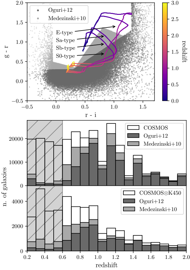
Figure C1. Top panel: (r-i) vs (g-r) diagram. We show the selections discussed in this article, following previous complementary works (Equations 14 and C1, Oguri et al. 2012; Medezinski et al. 2010, respectively). We additionally show the evolving tracks of spiral, lenticular and elliptical galaxies in the (g-r) -CC plane obtained using the GALEV code (Kotulla et al. 2009). Bottom panels: COSMOS (Ilbert et al. 2009) and COSMOS@K450 photometric redshift distributions for the full samples and for their dedicated (g-r) -CC selections. The shaded region highlights the contamination area, which corresponds to the cluster redshift range [0.1, 0.6] covered in Section 3.3.2.
