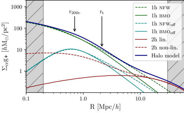
Figure 4. The halo model (blue) is composed of the BMO halo mass profile (thick green, Baltz et al. 2009), its off-centered contribution (thick cyan, Johnston et al. 2007b) and the second term derived from the linear matter power spectrum (thick red, Eisenstein & Hu 1999). For comparison, we show the centered / off-centered NFW mass profile (dashed green / cyan, Navarro et al. 1997) and the surrounding matter term with a non-linear power spectrum (dashed red, Takahashi et al. 2012). The density profile is computed in this example for a halo at z_1 = 0.2 with a total mass M_{200c} = 10^{14} M_{\odot}/h , a concentration c_{200c} = 4 and a bias set at b_h = 1 (with \sigma_8 = 0.83 ). The variance and the fraction of an off-centered population contribute to the profile with \sigma_{\text{off}} = 0.25 \text{ Mpc}/h and f_{\text{off}} = 0.25 . Finally, the reduced shear is given for an effective source redshift z_s = 1 , while the non-shaded area reveals the range allowed by the stacked WL analysis.
