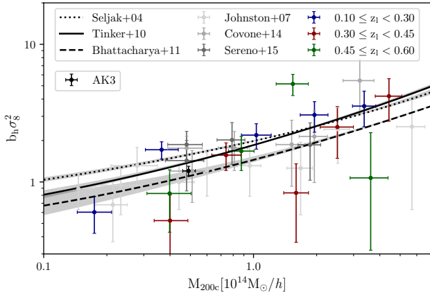
Figure 9. Halo bias-mass relation for the full catalog (black) and for the low (blue), intermediate (red) and high (green) redshift bins. The results on the halo bias are compared with calibrated data from a stacked WL analysis on SDSS and CFHTLenS galaxy clusters (Johnston et al. 2007a; Covone et al. 2014; Sereno et al. 2015b). Theoretical relations are derived from Seljak & Warren (2004); Tinker et al. (2010); Bhattacharya et al. (2011) and respectively displayed as dotted, thick and dashed lines. These functions are computed within their confidence interval using the values of \sigma_8 reported in Table 3.
