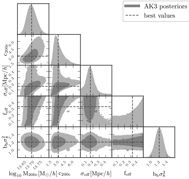
Figure 5. Posterior distributions arising from the halo model and the density profile derived in this study. The median of the marginalized distribution of the mass, concentration, off-centering parameters and bias are displayed as dashed lines. The 2D posterior distributions also show the 68% and 95% confidence regions in shaded grey regions.
