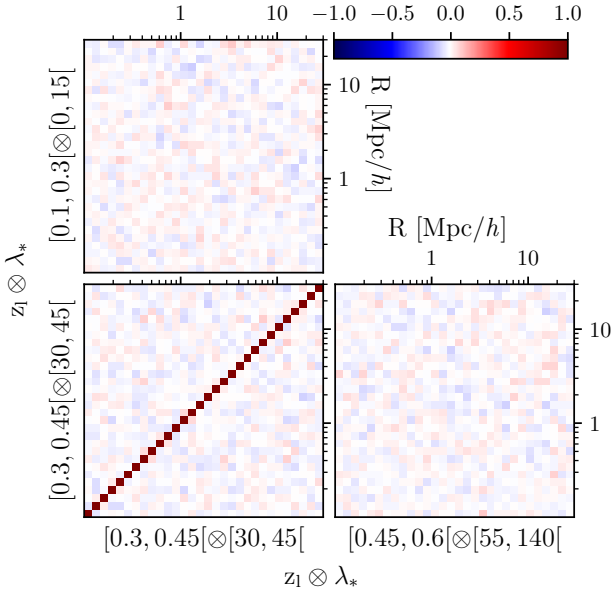
Figure A1. Bootstrap correlation matrix of \overline{\Delta\Sigma} , computed from z_1 \otimes \lambda_* selected bins. Here, we investigate the bin [0.3, 0.45] \otimes [30, 45[ correlated with itself (bottom left panel), with the bin [0.1, 0.3] \otimes [0, 15[ (top panel) and with the bin [0.45, 0.6] \otimes [55, 140[ (bottom right panel). The statistical uncertainty is mainly provided by the diagonal terms, while the off-diagonal terms are nearly consistent with zero, suggesting that radial and redshift-richness bins do not correlate.
