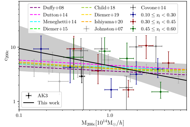
Figure 8. The relation between the mass and the halo concentration for the full catalog (black) and for the low (blue), intermediate (red) and high (green) redshift bins. The results on the concentration are compared with calibrated data from a stacked WL analysis on SDSS and CFHTLenS galaxy clusters (Johnston et al. 2007a; Covone et al. 2014). The thick black line reports the best estimate of the linear regression for Equation (37) with its 1\sigma confidence region. The relation is contrasted with results given by different theoretical analyses (Duffy et al. 2008; Dutton & Macciò 2014; Meneghetti et al. 2014; Diemer & Kravtsov 2015; Child et al. 2018; Diemer & Joyce 2019; Ishiyama et al. 2020).
