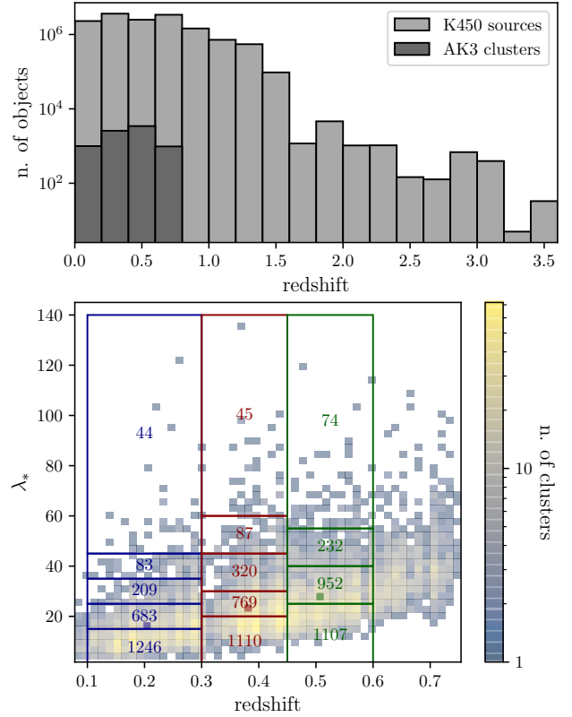
Figure 1. Top panel: Redshift distributions of AK3 clusters (dark gray) and K450 galaxies (light gray). Bottom panel: AK3 clusters in the redshift-richness plane with SNR \geq 3.5 . Colored rectangles correspond to the redshift-richness bins used in the following analysis (see Section 3.4); the number of clusters enclosed in each bin is displayed. Single colored squares show the mean values in each redshift bin computed as in Equation (17).
