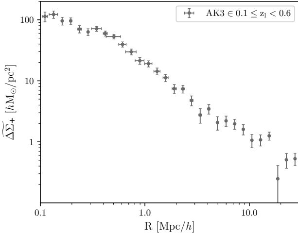
Figure 3. The stacked matter density profile of AK3 clusters with 0.1 \leq z_1 < 0.6 . The signal is computed assuming the combined selections given in Equation (15). Horizontal and vertical bars are derived from Equation (11).
