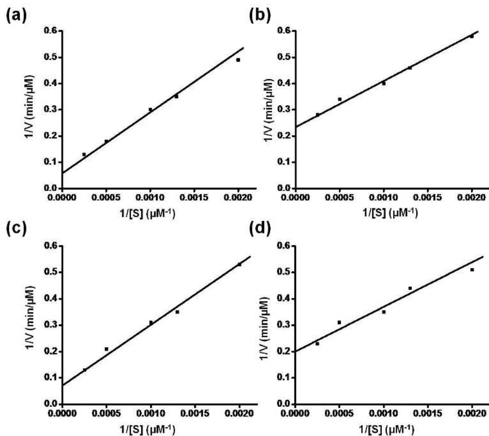
Figure 8: Lineweaver-Burk plot for hydrolysis of p -nitrophenyl butyrate (PNPB) catalyzed by (a) ferric ion based hydrogel, (b) aggregated AM1 and hydrolysis of p -nitrophenyloctanoate (PNPO) catalyzed by (c) ferric ion based hydrogel, (d) aggregated AM1
