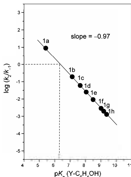
Figure 4. Plot of \log k_2/k_{-1} vs. \text{p}K_{\text{a}} of the conjugate acids of the leaving aryloxides for reactions of 1a-h with piperidine in 80 mol % H 2 O/20 mol % DMSO at 25.0 ± 0.1 °C. The identity of points is given in Table 2.
