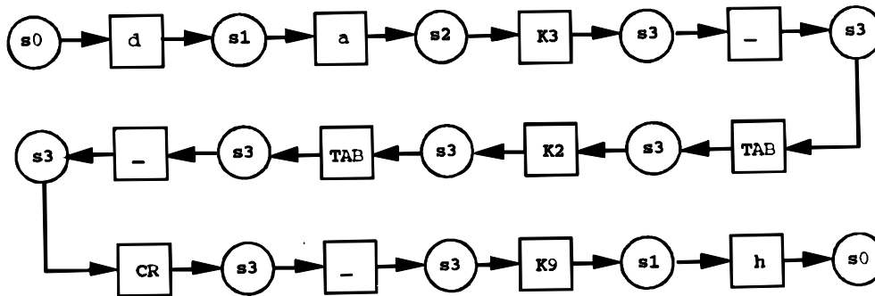
Figure 1. A sequence generated by a user operating a relational database program (see Rauterberg 1992a). The whole process of the shown example is based on 12 transitions (#AT) and 12 + 1 = 13 states (#AS). The representation of this process is given in a complete \dots \rightarrow (\text{state}) \rightarrow [\text{transition}] \rightarrow (\text{state}) \rightarrow \dots description. Legend: (s0) = main menu state, (s1) = module 'data' state, (s2) = routine 'browse' state, (s3) = wrong input state; [_] = ascii key 'BLANK', [a] = ascii key 'a', [d] = ascii key 'd', [h] = ascii key 'h', [CR] = carriage return, [K2] = function key 'F2', [K3] = function key 'F3', [K9] = function key 'F9', [TAB] = tabulator key.
