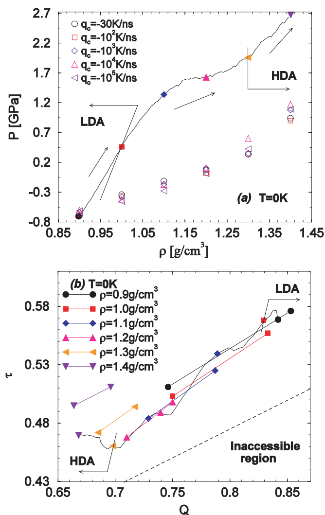
Figure 28. (a) Comparison of the location in the P - \rho plane of the glasses at T = 0\text{ K} obtained by isothermal compression of LDA (black line, filled symbols) and by isochorically cooling the liquid at different densities and cooling rates (open symbols). (b) Location in the Q - \tau plane. Results from computer simulations using the SPC/E model (from [218]).
