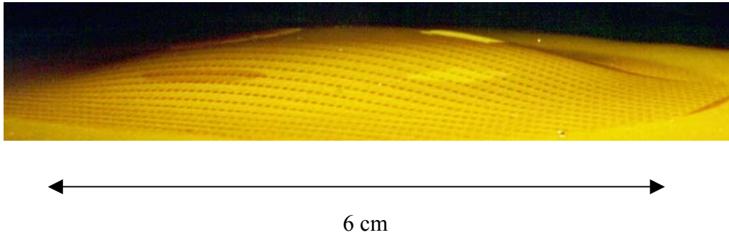
Figure 1. Polyimide foil with a-Si/SiN x islands after deformation to a spherical cap shape with a ~66° field-of-view.
