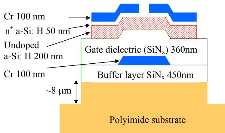
Figure 2. Cross-section of the TFT structure.
