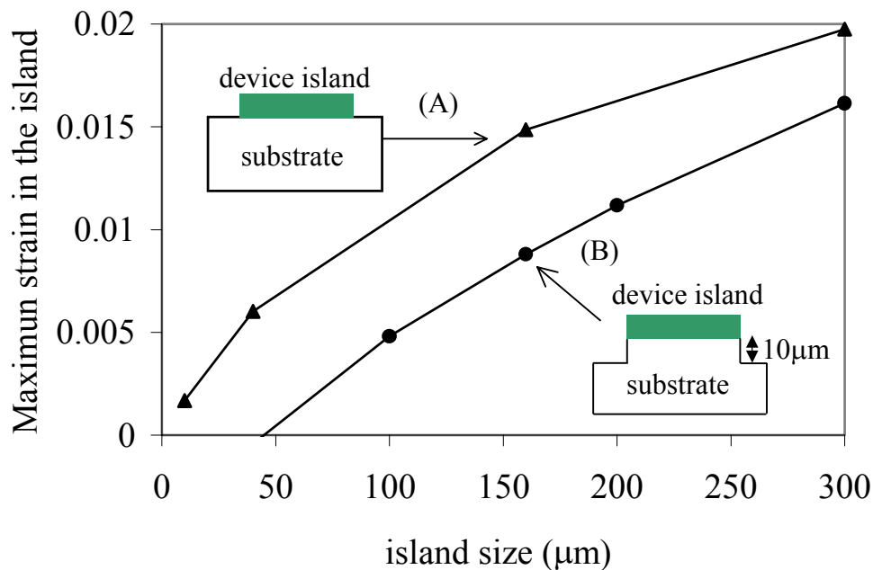
Figure 7. Finite element analysis of the maximum strain in the island as a function of the island size for 0.5 \mu\text{m} -thick circular silicon islands on 50- \mu\text{m} -thick polyimide substrate after the substrate is deformed with 6% strain. (A): Device island on uniform polyimide substrate. (B): Device island on polyimide mesa substrate.
