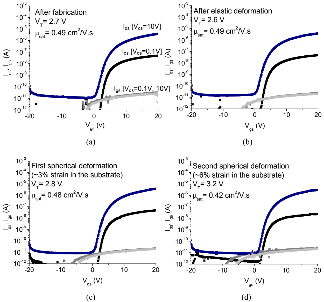
Figure 5. TFT characteristics. The device shown here is on a 40\ \mu\text{m} \text{SiN}_x island on with gate length L = 4\ \mu\text{m} and gate width W = 14\ \mu\text{m} . (a) After fabrication. (b) After elastically deformed into a spherical dome with \sim 1.5\% strain in the substrate, and then released to relax the substrate to its original planar form. (c) After plastic deformation into a 50^\circ field-of-view spherical dome ( \sim 3\% strain in the substrate). (d) After plastic deformation into a 66^\circ field-of-view spherical dome ( \sim 6\% strain in the substrate). The TFT is still well behaved with comparable electric performance after each deformation step.
