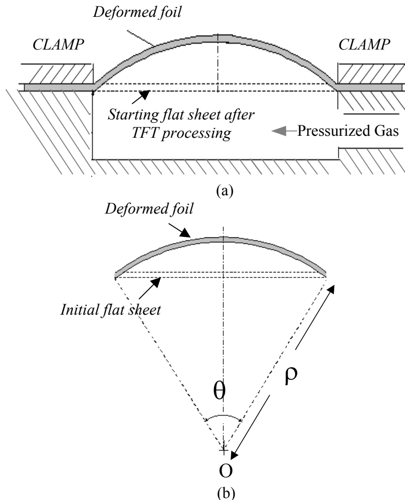
Figure 3. (a) Design of the apparatus used for deforming thin foil substrates. (b) Schematic cross-section of the foil before and after deformation. Point "O" is the resulting center of curvature of the cap, and subtended angle \theta is the field-of-view [5].
