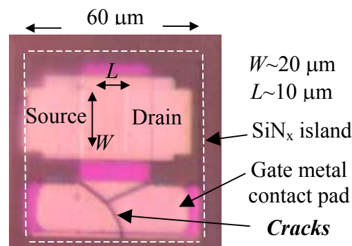
Figure 4. Optical micrograph of fractured 60\ \mu\text{m} device island after deformation to a 50^\circ field-of-view spherical dome. The fracture begins at the gate contact pad region.
