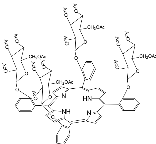
Figure 1. Structure of glycosylated porphyrin.
