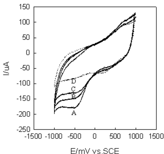
Figure 2. Cyclic voltammograms obtained with a MnT( o -glu)TTCl-modified electrode after incubation in MTZ solutions of concentration (A): 5 \times 10^{-4} M/L, (B): 1 \times 10^{-5} M/L, (C): 5 \times 10^{-7} M/L, and a unmodified one incubated in 5 \times 10^{-4} M/L MTZ (D).
