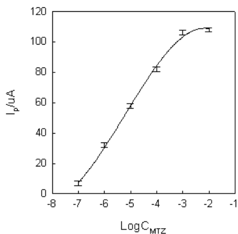
Figure 5. Calibration graph for the MTZ sensor obtained with the MTZ sensor incubated in MTZ solutions of different concentrations followed by voltammetric measurements. Operating potential: - 408 mV vs. SCE.
