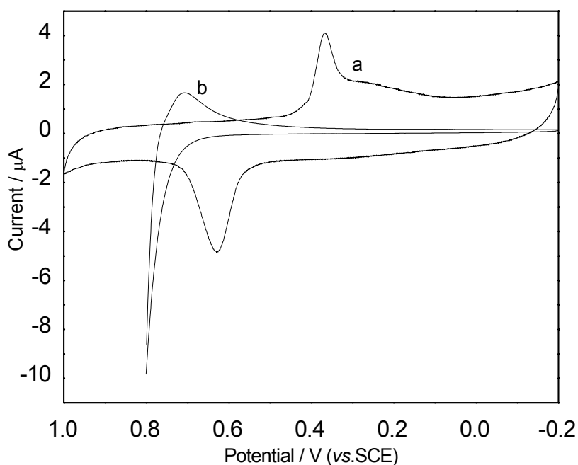
Figure 2. Cyclic voltammograms at (a) silver nanoparticles modified electrode and at silver micro-disk electrode (b) in 0.1 mol/L PBS (pH 6.0); scan rate: 80 mV/s; scan from 1.0 (a) or 0.8 (b) to -0.2 V.
