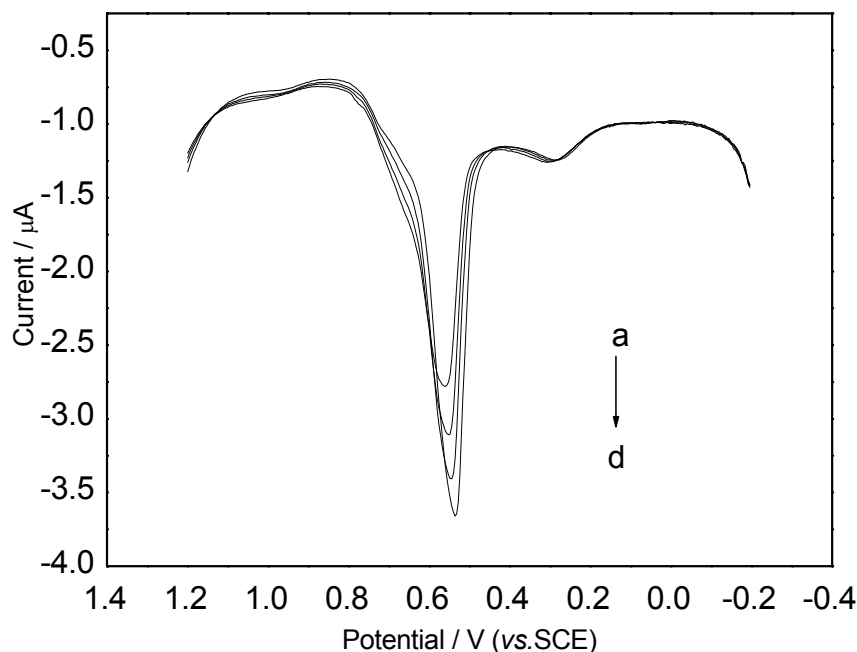
Figure 5. DPV of \text{SCN}^- on Ag nanoparticles modified electrode. The concentration of \text{SCN}^- : (a) 9; (b) 12; (c) 15; (d) 18 \mu\text{mol/L} .
