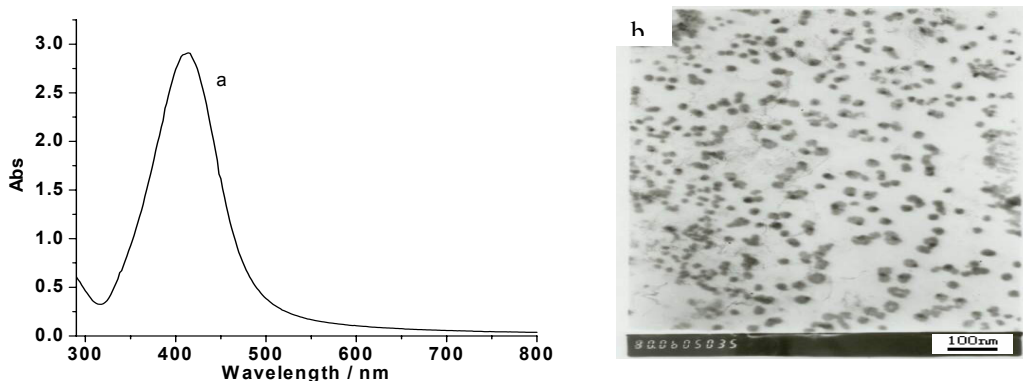
Figure 1. (a) UV-vis spectrum of the silver nanoparticles capped by oleate and (b) TEM of Ag nanoparticles.
