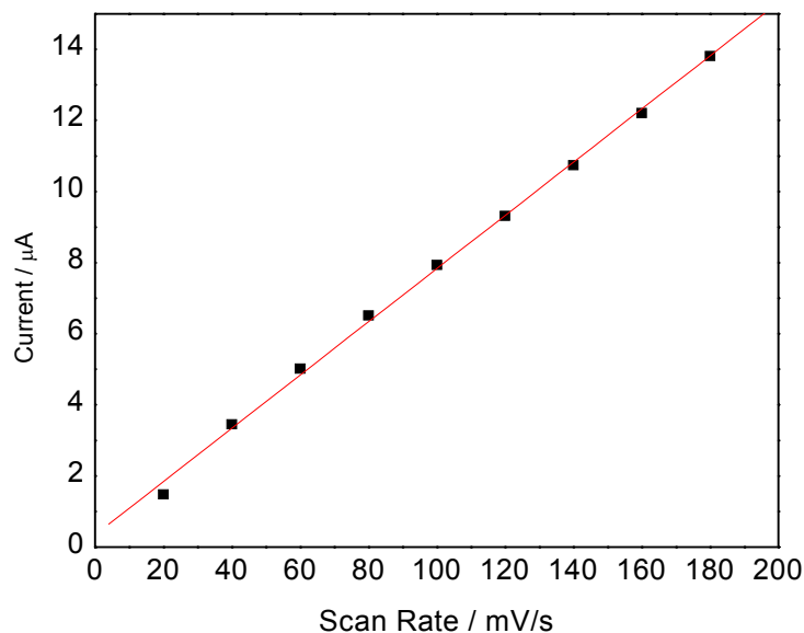
Figure 4. Relationship between scan rate and oxidation peak current in 1.5 \times 10^{-5} mol/L \text{SCN}^- at the Ag nanoparticles modified GC electrode in 0.1 mol/L PBS (pH 6.0).
