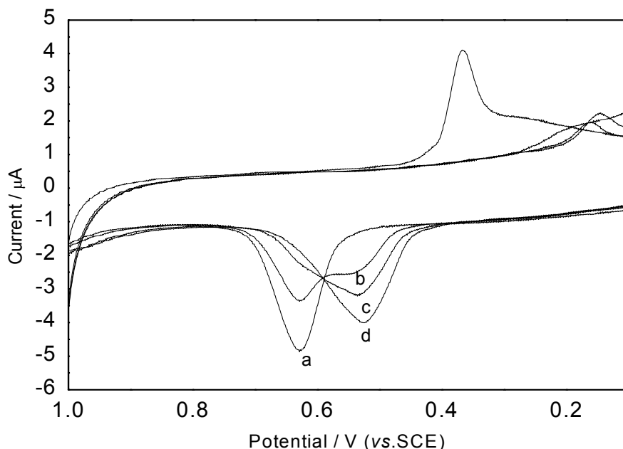
Figure 3. CV curve of \text{SCN}^- of different concentrations at silver nanoparticles modified electrode. (a) 0; (b) 5.0 \times 10^{-5} ; (c) 10 \times 10^{-5} ; (d) 15 \times 10^{-5} mol/L \text{SCN}^- in 0.1 mol/L PBS (pH 6.0); scan rate: 80 mV/s.
