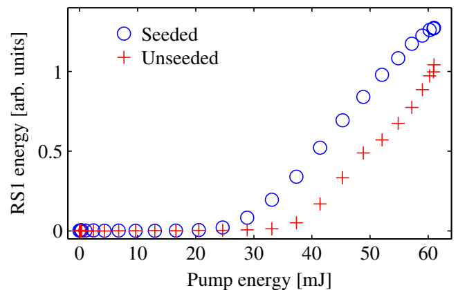
FIG. 2 (color online). Rotational-Stokes 1 growth at 549 nm in hydrogen at 760 torr as a function of pump pulse energy for seeded (blue circles) and unseeded (red crosses) cases. Stokes growth is more efficient when a 12 \mu\text{J} seed is used.
