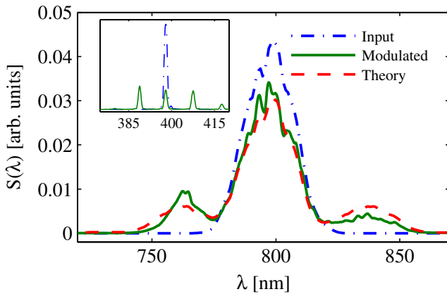
FIG. 3 (color online). The 800 nm probe spectrum after propagation through the seeded hydrogen gas at 1500 torr with (solid green line) and without (dash-dotted blue line) the pump. MPM broadens the probe spectrum when the pump is on. The theory plot (dashed red line) is generated by numerical solution of the equations describing the one-dimensional Raman field-matter interaction. Inset: 400 nm probe spectrum with (solid green line) and without (dash-dotted blue line) the pump.
