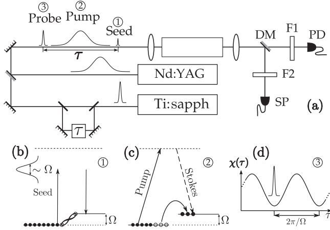
FIG. 1. Diagram showing the experimental setup (a) and field-matter interactions (b,c,d) for phase-stable MPM. A Ti:sapphire chirped pulse amplifier laser produces a weak seed pulse and a delayed probe pulse; a Nd:YAG laser generates the pump pulse. (b) The seed excites a rotational coherence by ISRS. (c) The coherence is enhanced using a phase-independent pump pulse. (d) The probe pulse is spectrally broadened by MPM.
