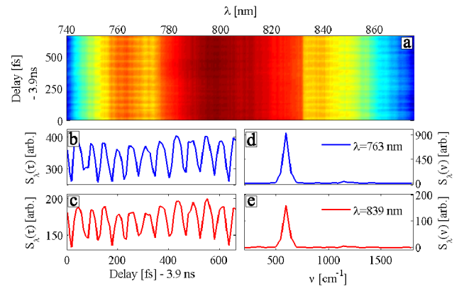
FIG. 4 (color online). (a) Probe spectrum as a function of delay relative to the seed pulse from an initial delay of 3.9 ns. Line outs from the probe spectrum at \lambda = 763 \text{ nm} (b) and \lambda = 839 \text{ nm} (c). Peaks at \Omega in the Fourier spectrum of the line outs (d), (e). The delay-dependent oscillations at \Omega demonstrate phase coherence of the excitation with respect to the probe pulse.
