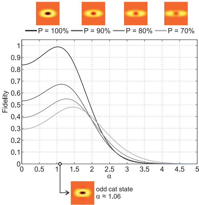
FIG. 3. (Color online) Fidelity between an ideal cat state |\kappa_-(\alpha)\rangle and the small-amplitude cat states obtained from the squeezed vacuum \xi_p = -3 dB at four squeezing purities \mathcal{P} (marked in decreasing darkness of gray): 100%, 90%, 80%, and 70%. The Wigner functions of the PSSVs corresponding to these four purities are shown at the top. As a reference for what the “ideal” output ought to look like, the Wigner function of the state |\kappa_-(1.06)\rangle , which has the highest fidelity with the PSSV obtained from pure squeezing, is shown at the bottom. The transmission of the subtraction beam splitter is set at 99%.
