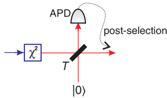
FIG. 1. (Color online) Setup for the generation of approximate small-amplitude odd cat states. A squeezed vacuum, represented here by the pumping of a \chi^2 nonlinear medium, is partially reflected onto an “on-off” photon detector such as an avalanche photodiode (APD). Upon the reflection of at least one photon from the squeezed vacuum, a state that likens the squeezed single photon is prepared in the limit of unit transmission T \rightarrow 1 .
