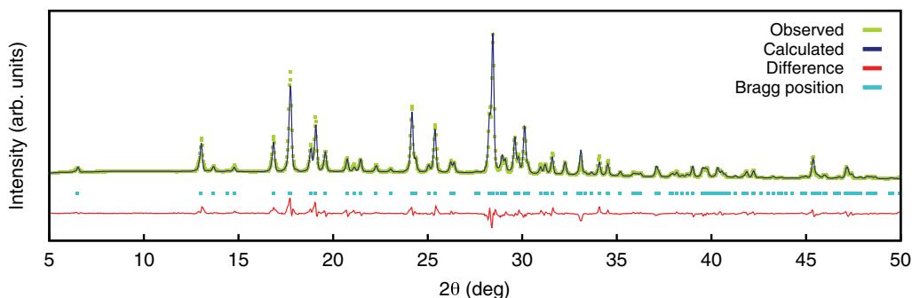
FIG. 3. Results from a least-squares fit using the Rietveld method: experimental powder diffraction pattern (green); simulated diffraction pattern using the Rietveld method (dark-blue); difference between the observed and calculated intensities (red), and corresponding Bragg positions (blue).
