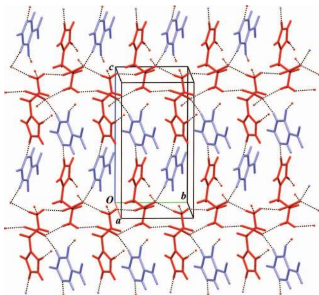
FIG. 2. Guest-host structure of L-His + 5NU - . The anions (blue) are encapsulated between the cationic layers (red) in a polar herringbone motif along the b axis (Mercury 2.4 (Ref. 43)).
