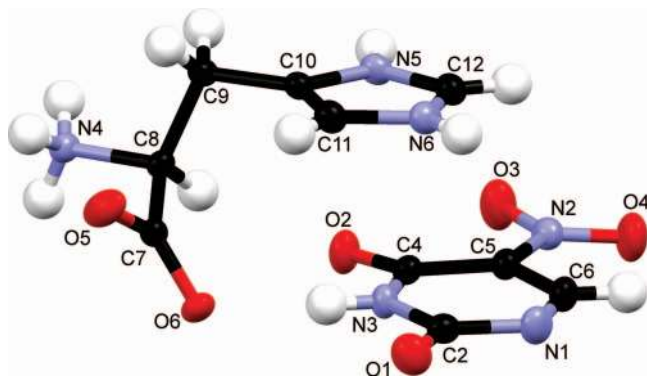
FIG. 1. Asymmetric unit of L-His + 5NU - . The displacement ellipsoids are drawn at the 50% probability level (Mercury 2.4 (Ref. 43)).
