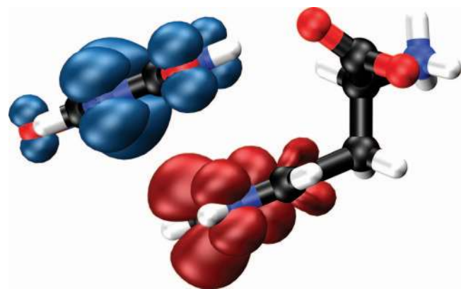
FIG. 4. Difference density plot (isovalue 0.004) between ground and excited state ( S_1-S_0 ) of L-His + 5NU - obtained from a TD-DFT (X3LYP/6-311++G**) calculation. Blue indicates positive values and red negative values.
