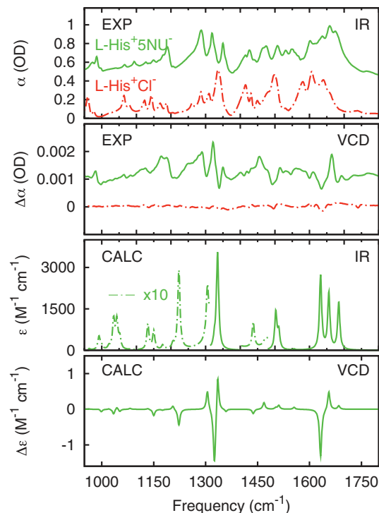
FIG. 5. Upper panels: Fourier-transform infrared (FTIR) and VCD spectra of L-His + 5NU - and L-His + Cl - obtained with KBr pellet technique. Lower panels: Calculated IR and VCD spectra for L-His + 5NU - using DFT/X3LYP/6-311++G** level of theory. Some of the peaks are scaled for clear comparison with the experimental spectrum.
