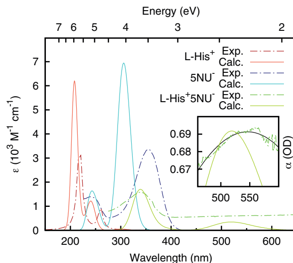
FIG. 6. Optical absorption spectra of L-His + (dashed-red), obtained with an acidic H 2 O solution; 5NU - (blue), obtained from a basic H 2 O solution; and the salt: L-His + 5NU - , obtained with a 1 mm thin-film deposited in a 1 mm thick CaF 2 window. Calculated spectra were obtained at the TD-DFT/X3LYP/6-311++G** level of theory. Inset: enhanced range of the experimental spectrum of the thin-film of the salt to elucidate the presence of the band at 550 nm. Due to low intensity of the bands of the ionic salt, the extinction coefficients for the chromophores are scaled in intensity for clear comparison.
