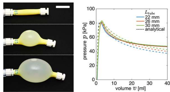
Fig. S3. Evolution of pressure ( p ) as a function of the supplied volume ( v ) for three latex tubes characterized by L_{tube} = 22, 26, and 30 mm as measured in experiments (solid lines) and predicted by the analytical model (dashed lines). Snapshots of a tube characterized by L_{tube} = 22 mm at v = 0, 20, 40 mL are shown on the left. (Scale bar: 10 mm.)
