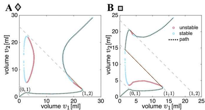
Fig. 56. Numerical results for two combined soft actuators with n=2 . (A) Relation between the individual volumes of the segments for a soft actuator with (L_{braid}, L_{tube}) = (48, 30) and (50, 20) mm. (B) Relation between the individual volumes of the segments for a soft actuator with (L_{braid}, L_{tube}) = (44, 30) and (48, 26) mm.
