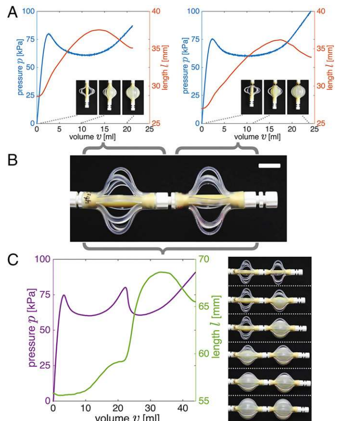
Fig. 2. (A) Evolution of pressure ( p ) and length ( l ) as a function of the supplied volume ( v ) for two fluidic segments characterized by (L_{braid}, L_{tube}) = (46, 20) and (46, 22) mm. Snapshots of the fluidic segments at v = 0, 10, 20 and v = 0, 12, 24 mL are shown as Insets , respectively. (B) The two fluidic segments are connected to form a new, combined soft actuator. (C) Evolution of pressure ( p ) and length ( l ) as a function of the supplied volume ( v ) for the combined actuator. Snapshots of the combined actuator at v = 0, 9, 18, 27, 36, 45 mL are shown as Insets .
