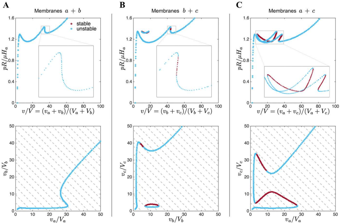
Fig. S2. Response of two interconnected spherical membranes upon inflation. The response of the individual membranes is shown in Fig. S1. The equilibrium states and their stability have been obtained numerically. The pressure–volume relation and the relation between the volume of the individual membranes are shown for systems comprising (A) membranes a and b , (B) membranes b and c , and (C) membranes a and c .
