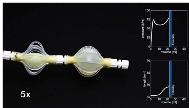
Movie S3. Inflation of a combined soft actuator. Inflation of a combined soft actuator consisting of two interconnected fluidic segments, characterized by (L_{braid}, L_{tube}) = (46, 20) and (46, 22) mm. In the experiment, we inflated the segment with water at a rate of 20 mL/min. At v = 23 ml an instability at constant volume is triggered, causing a sudden increase in length, internal volume flow, and pressure drop.
