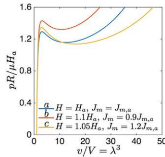
Fig. S1. Relation between the pressure and volume for three different hyperelastic spherical membranes upon inflation.
