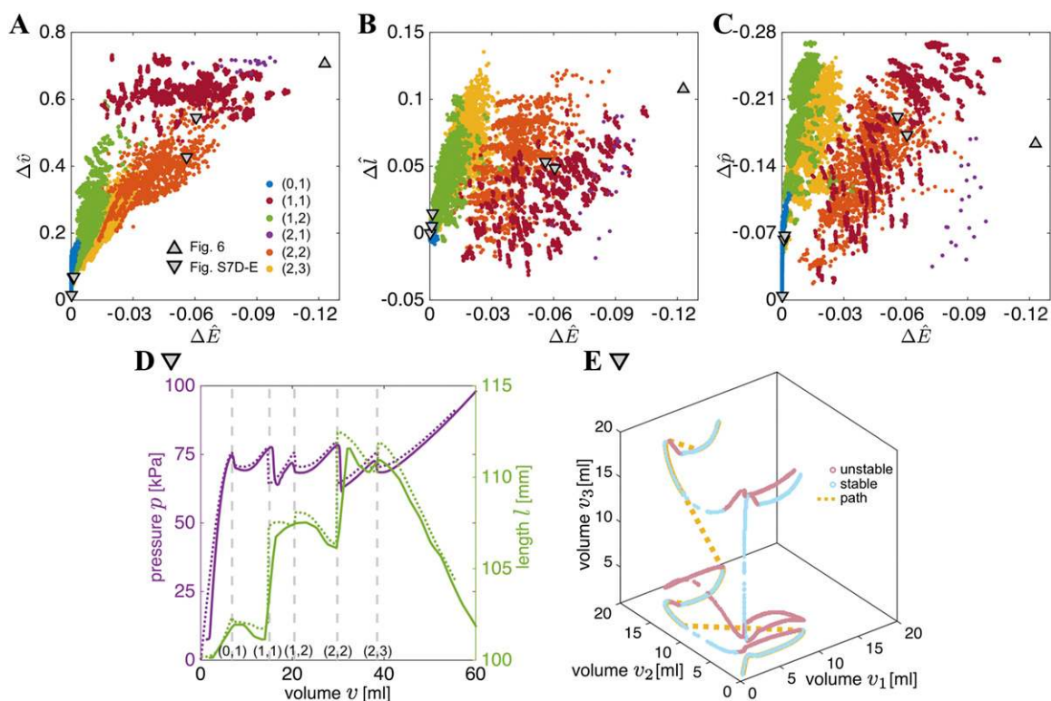
Fig. S7. (A–C) \Delta \hat{v} , \Delta \hat{l} and \Delta \hat{p} versus the normalized change in energy \Delta \hat{E} for all state transitions that occur in the 7,140 combined soft actuators comprising n=3 fluidic segments. Blue, red, green, purple, orange, and yellow markers correspond to (0, 1), (1, 1), (1, 2), (2, 1), (2, 2), and (2, 3) transitions, respectively. (D) Experimental (solid line) and numerical (dashed line) evolution of pressure and length as a function of the supplied volume for a soft actuator with n=3 , characterized by (L_{\text{braid}}, L_{\text{tube}}) = (40, 28) , (44, 22) , and (48, 26) mm. (E) Numerically determined relation between the individual volumes of the three segments.
