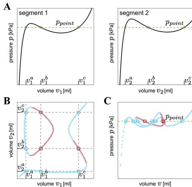
Fig. 55. Numerical procedure to determine the equilibrium configurations for a combined actuator with n=2 . (A) We identify the volumes of each segment that correspond to a given value of pressure (in this case p_{point} ). (B) We find all corresponding equilibrium configurations for the combined actuator by combining all those volumes. (C) Because v=v_1+v_2 , we can also identify all equilibrium points in the pressure–volume curve for the combined actuator.
