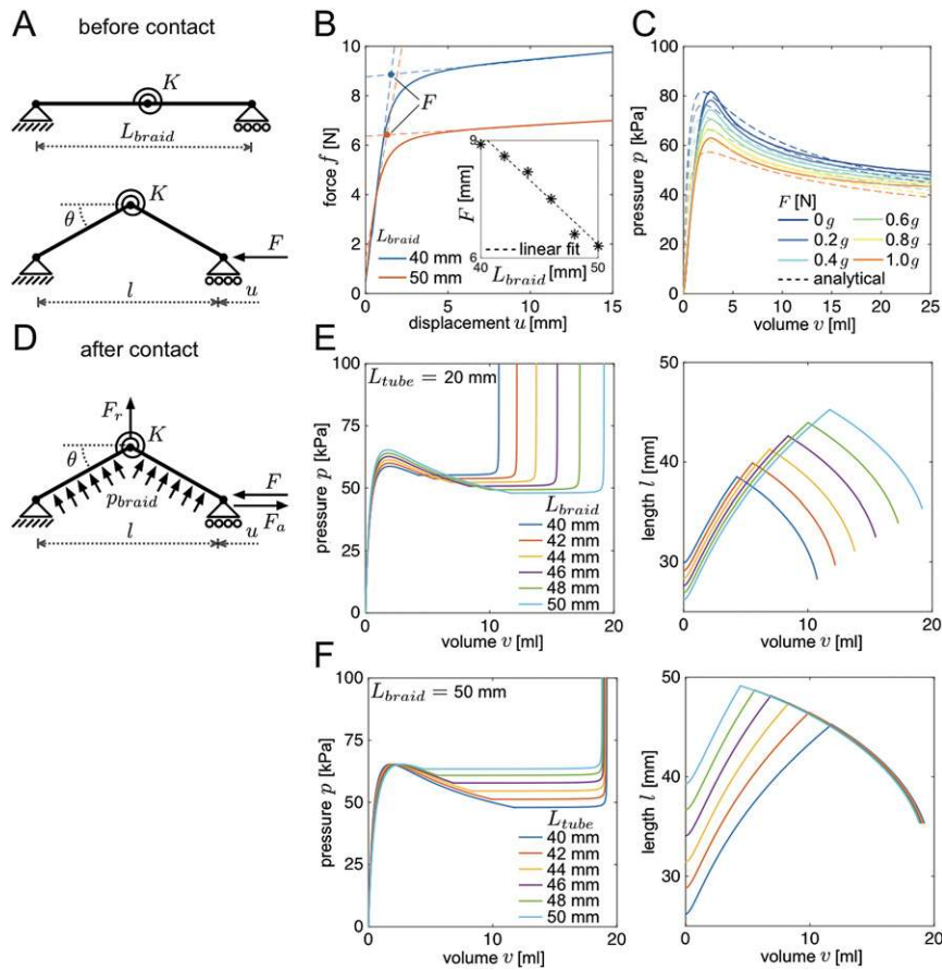
Fig. S4. Analytical prediction of the response of individual fluidic segments. (A) Diagram of the braids before contact with the membrane (i.e., v < v_{braid} ). (B) Experimentally obtained force-displacement relation for braids with L_{braid} = 40 - 50 under uniaxial compression. The Inset shows the critical force, F , measured from experiments. (C) Evolution of pressure ( p ) as a function of the supplied volume ( v ) for a latex tube subjected to an axial force F = 0 - 1g ( g denoting the gravitational acceleration). Continuous and dashed lines correspond to experimental data and analytical predictions, respectively. (D) Diagram of the braids after contact with the membrane. (E) Predicted response for six segments characterized by L_{tube} = 20 mm and L_{braid} = 40 - 50 mm. (F) Predicted response for six segments characterized by L_{tube} = 20 - 30 mm and L_{braid} = 50 .
