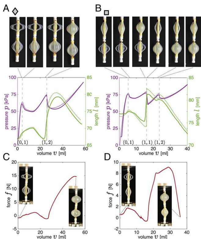
Fig. 5. (A and B) Experimental (solid lines) and numerical (dashed lines) pressure–volume curves for two soft actuators comprising n=2 fluidic segments. (A) Results for a combined actuator with (L_{\text{braid}}, L_{\text{tube}}) = (48, 30) and (50, 20) mm. The transitions for this actuator are highlighted by diamond markers in Fig. 4. Snapshots of the combined actuators 0.5 mL before and after each state transition (at v = 4, 26 mL) are also shown. (B) Results for a combined actuator with (L_{\text{braid}}, L_{\text{tube}}) = (44, 30) and (48, 26) mm. The transitions for this actuator are highlighted by square markers in Fig. 4. Snapshots of the combined actuators 0.5 mL before and after each state transition (at v = 5, 16, 24 mL) are also shown. Experimentally measured exerted force as a function of the supplied volume for a combined actuator with (C) (L_{\text{braid}}, L_{\text{tube}}) = (48, 30) and (50, 20) mm and (D) (L_{\text{braid}}, L_{\text{tube}}) = (44, 30) and (48, 26) mm with constrained ends.
