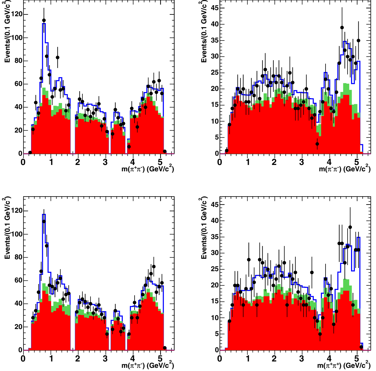
FIG. 4: Projection plots of the fit results for B^- \rightarrow \pi^- \pi^- \pi^+ and B^+ \rightarrow \pi^+ \pi^+ \pi^- onto the mass variables m_{\pi^+ \pi^-} and m_{\pi^- \pi^-} ( m_{\pi^+ \pi^+} ). The upper (lower) plots are for the B^- ( B^+ ) data sample. The data are the black points with statistical error bars, the lower solid red (dark) histogram is the q\bar{q} component, the middle solid green (light) histogram is the B\bar{B} background contribution, while the upper blue histogram shows the total fit result. The large dips in the spectra correspond to the charm vetoes.
