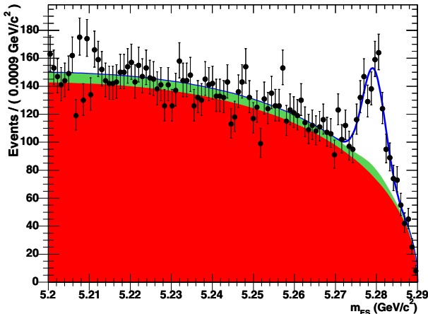
FIG. 1: The m_{ES} distribution along the \Delta E strip ( -65 < \Delta E < 55 MeV): the data are the black points with statistical error bars, the lower solid red (dark) area is the q\bar{q} component, the middle solid green (light) area is the B\bar{B} background contribution, while the upper blue line shows the total fit result.
