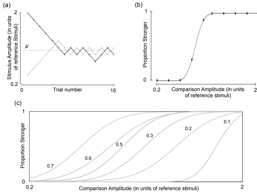
Fig. 2. (a) Staircase for one participants at \delta t = 0.5 s. The test converges to the amplitude at which the two signals feel identical, called the point of subjective equivalence. Here, \mu \approx 1.1 . (b) Psychometric curve fitted to the points for the same test. \mu is found at proportion stronger = 0.5. (c) General trend of the psychometric curves with time: psychometric curves for \delta t = 0.7, 0.6, 0.5, 0.3, 0.2 and 0.1 s.
