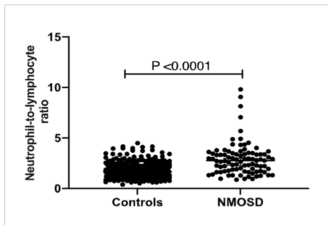
FIGURE 1 | Baseline NLR in HC and NMOSD patients. In patients, this NLR was taken during the first attack. The results of a two-tailed t-test are shown.
