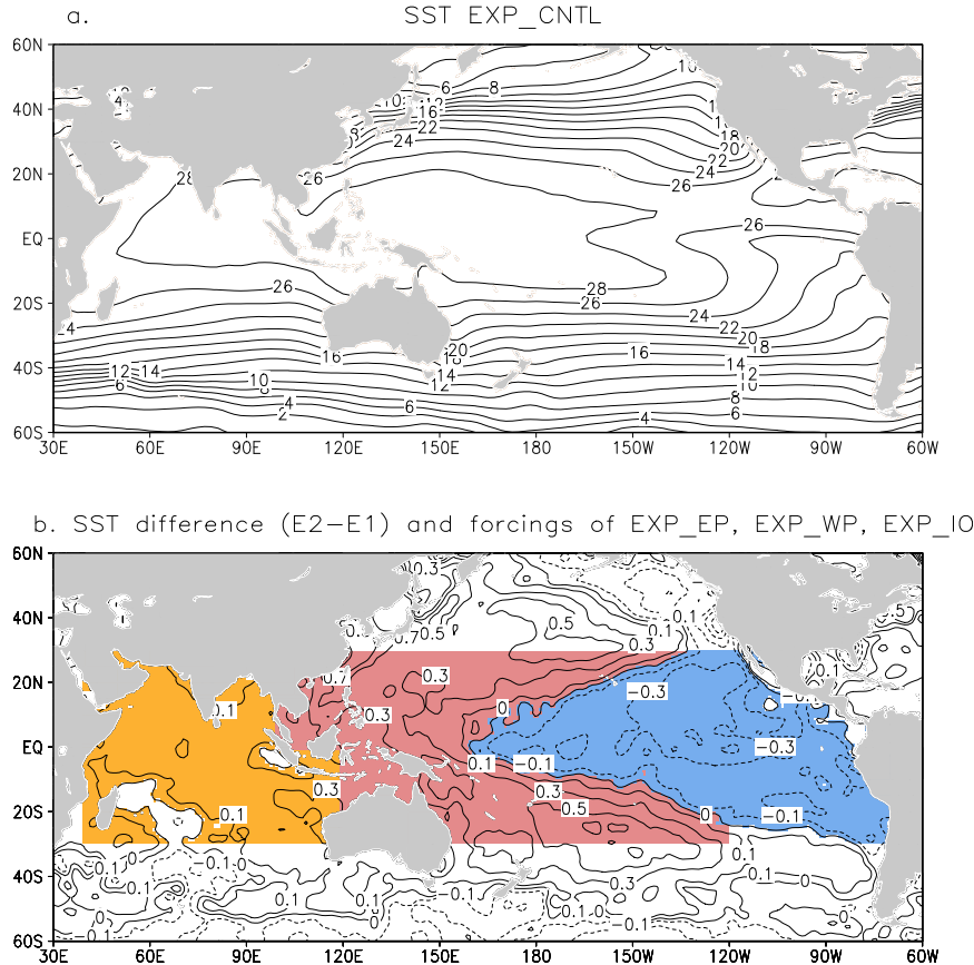
FIG. 7. (a) SSTs for the EXP_CNTL ( ^{\circ}\text{C} ). (b) Tropical SST anomalies (E2 minus E1, ^{\circ}\text{C} ) that are added to the SST in the EXP_CNTL to force the AGCM in the various experiments (blue for the EXP_EP, red for the EXP_WP, yellow for the EXP_IO, red and yellow for the EXP_WP+IO, and blue, red, and yellow together for the EXP_EP+WP+IO).
