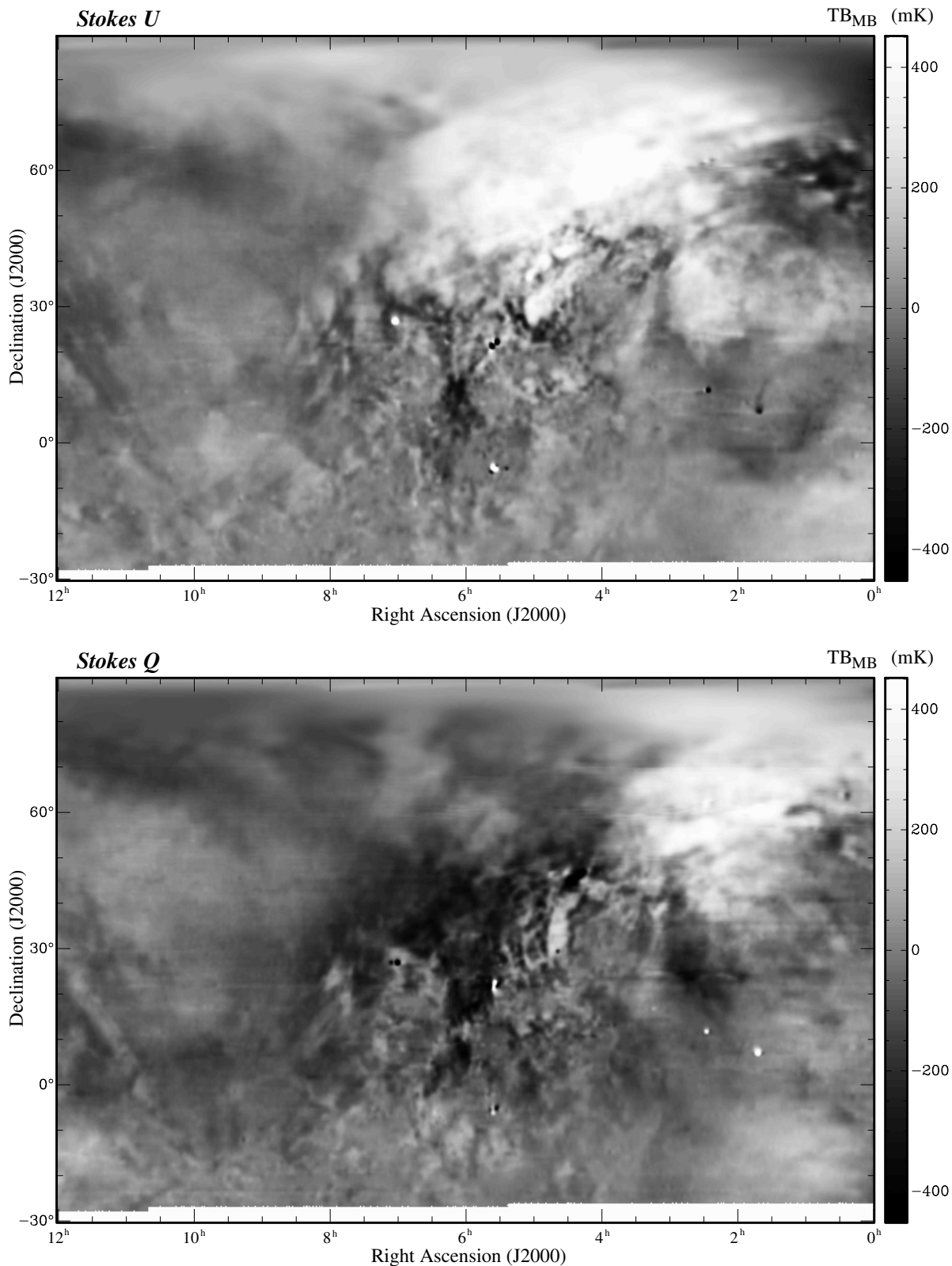
Fig. 9. Stokes U (top) and Q (bottom) in the right ascension interval from 0 h to 12 h in equatorial coordinates.
