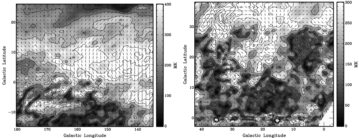
Fig. 11. The two maps of polarized intensity, with E-vectors of the polarized emission overlaid, show in greater detail part of the Fan-region ( left panel ) and the southern extension of the North-Polar Spur ( right panel ). In both maps depolarization caused by local H II-regions is apparent (NGC 1499: from l = 145^\circ to 170^\circ , b \lesssim -10^\circ ; and Sharpless 27: roughly 10^\circ in diameter, centered at l = 6^\circ and b = 23^\circ ). The synchrotron emission of the North-Polar spur seems to be depolarized at b \lesssim 25^\circ (from l = 30^\circ to 40^\circ ). In both maps contours of polarized intensity run from 0 mK to 800 mK in steps of 100 mK. Vectors are shown on a grid of 1.25^\circ .
