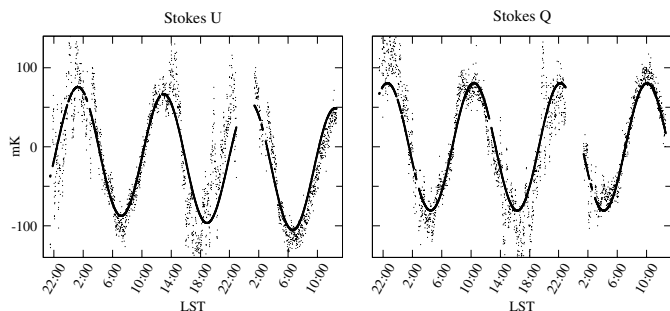
Fig. 3. A 1.5 day observation of the NCP, obtained on May 14th through May 16th, 2003. Shown are measurements made at daytime (20 h–11 h LST) and by night. The solid line shows a sine wave fitted to the data, taking a linear baseline into account. These data were calibrated in the following way: the electronic gain was corrected using the noise source (Sect. 4.3.1) and the Mueller matrix (Sect. 4.3.3) was applied.
