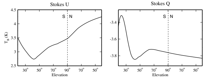
Fig. 5. Ground radiation profiles for Stokes U and Q determined on the basis of elevation scans. A possible explanation for the north-south asymmetry is given in the text.
