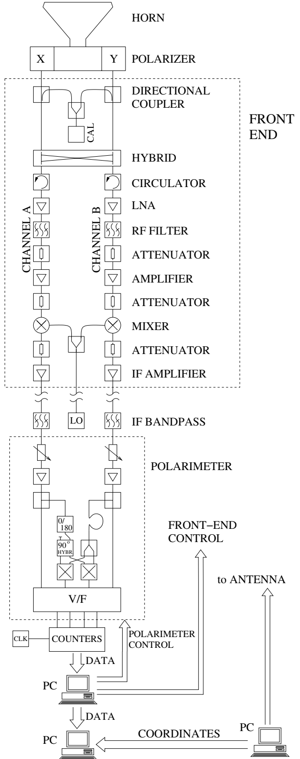
Fig. 1. Block diagram of the 1.4 GHz receiver and continuum backend of the DRAO 25.6-m telescope used for this survey. The polarimeter consists of two analog multipliers as indicated by cross symbols.
