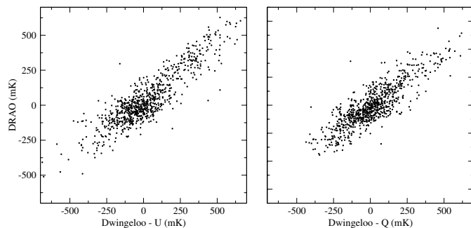
Fig. 7. Correlation of Stokes U ( left panel ) and Q ( right panel ) values from the DRAO survey with the Dwingeloo survey before adjusting the temperatures to the Effelsberg scale.
