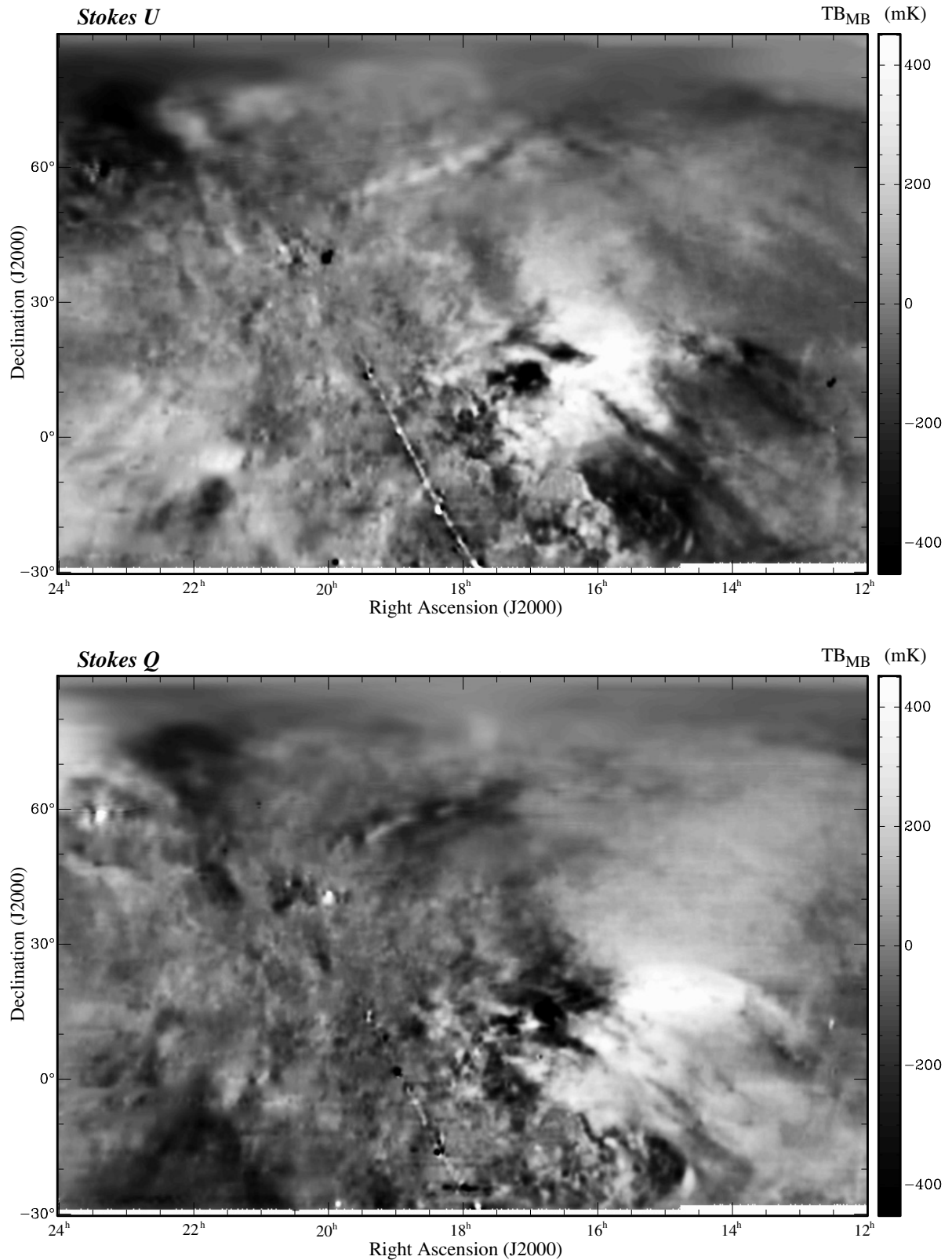
Fig. 8. Stokes U (top) and Q (bottom) in the right ascension interval from 12^{\text{h}} to 24^{\text{h}} in equatorial coordinates.
