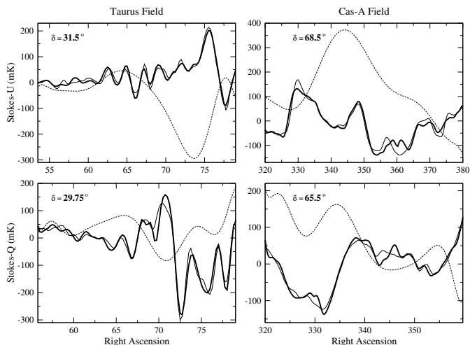
Fig. 6. Four scans through the two test regions used to establish the calibration of the survey relative to EMLS observations (thin solid lines), two from the Taurus complex ( left panels ) and two from the Cassiopeia-A region ( right panels ). DRAO survey data are drawn as thick solid lines. The large-scale emission missing from the EMLS data are shown as polynomials (whose characteristics were determined by an iterative technique and added to the EMLS data shown in this figure – see text) and are drawn as dashed lines. The declinations of the scans are indicated.
