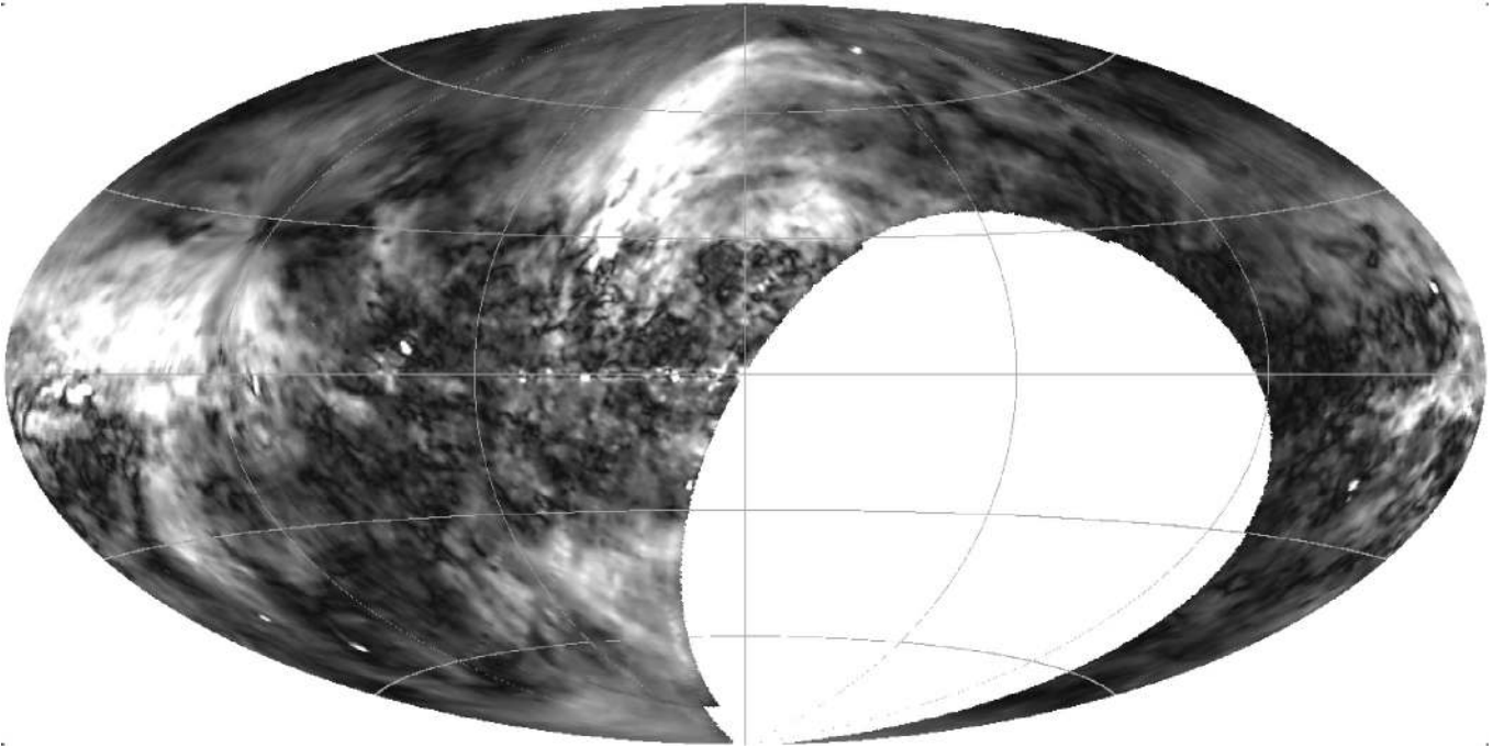
Fig. 10. Polarized intensity in Galactic coordinates. The projection center is at l = b = 0^\circ . The co-ordinate grid is in steps of 60^\circ in Galactic longitude and 30^\circ in Galactic latitude.
