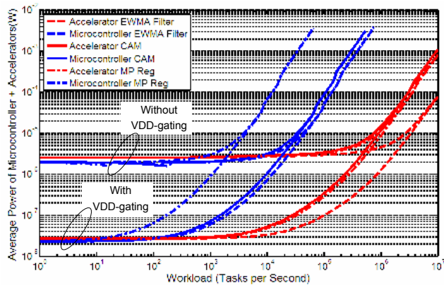
(b) Power vs. Workload
