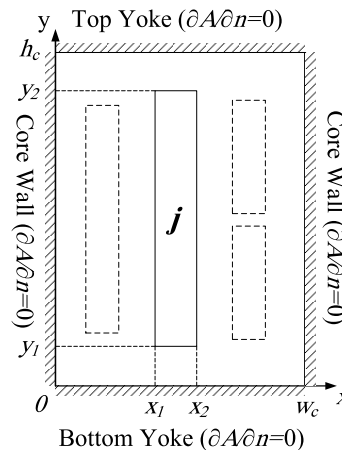
FIGURE 2. The geometry used for field analysis.
