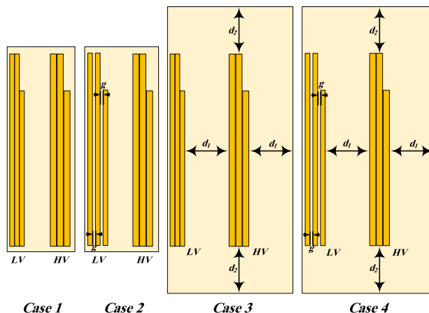
FIGURE 20. The different arrangements of the windings used in sensitivity analysis.
