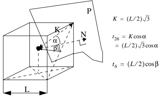
Figure 10. The 3D case (extended from Figure 7): L is the voxel's width, and K is the voxel's diagonal. N is the normal to the plane through the voxel's center, C . \alpha is the angle between N and K . \beta is the angle between N and the normal to the face of the voxel.
