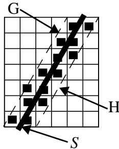
Figure 6. The plane S (solid line) and the two planes parallel to S at distance t , G and H (dashed lines). All voxels between G and H are included in the discrete representation of S .
