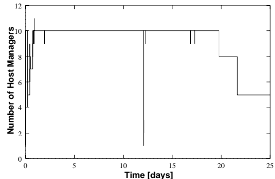
Figure 10: Host manager population changes on the Berkeley Network of Workstations over a 25 day period.
